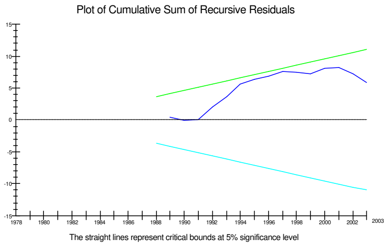
Figure 1: CUSUM TEST FOR EQUATION 12
