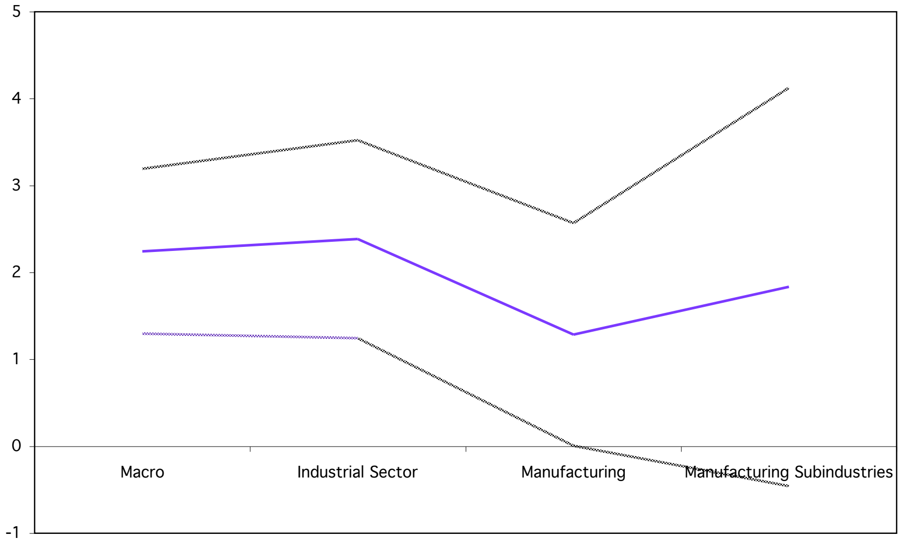
Coal-Gas Elasticities and 95% Confidence Interval
