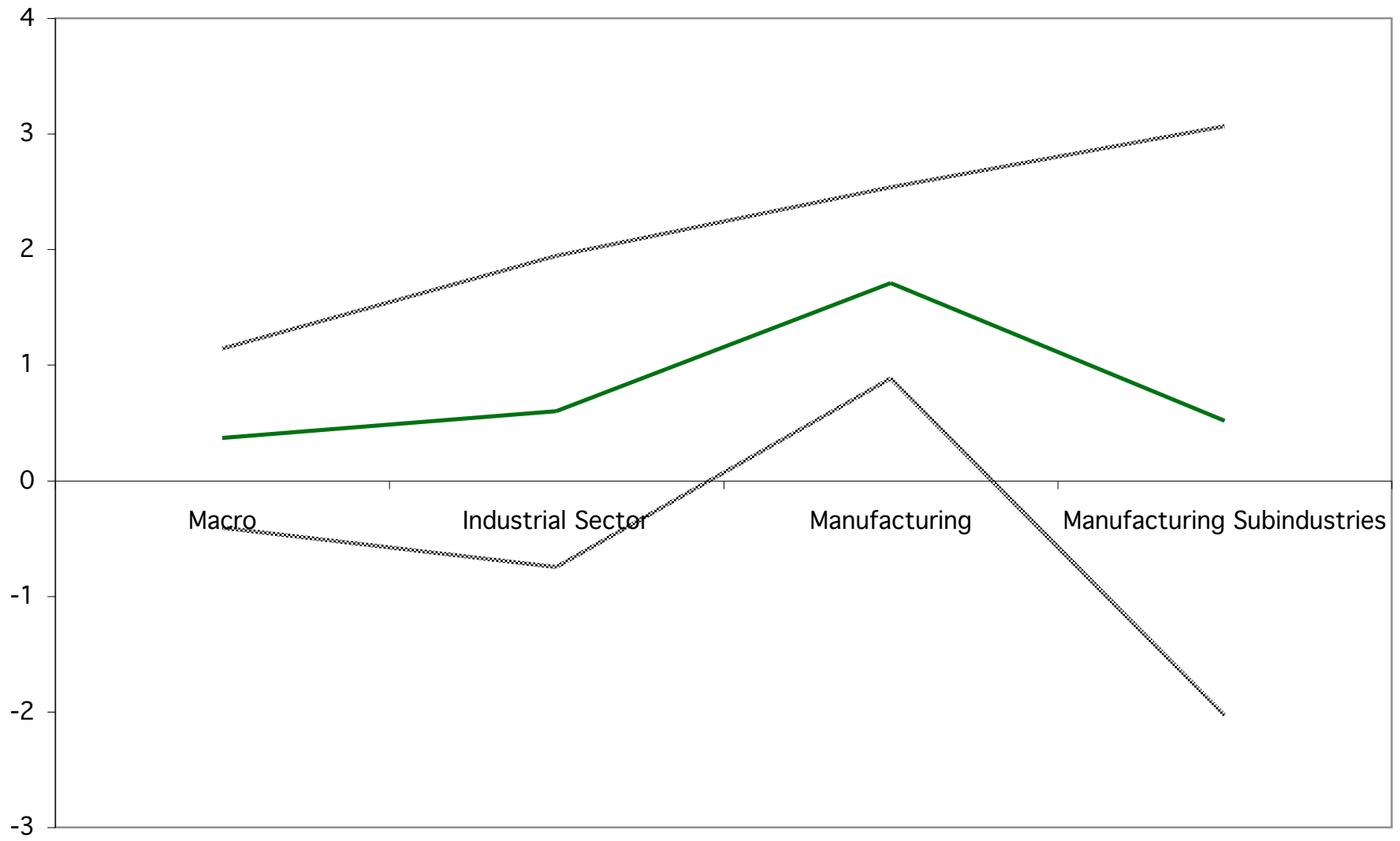
Oil-Gas Elasticities and 95% Confidence Interval
