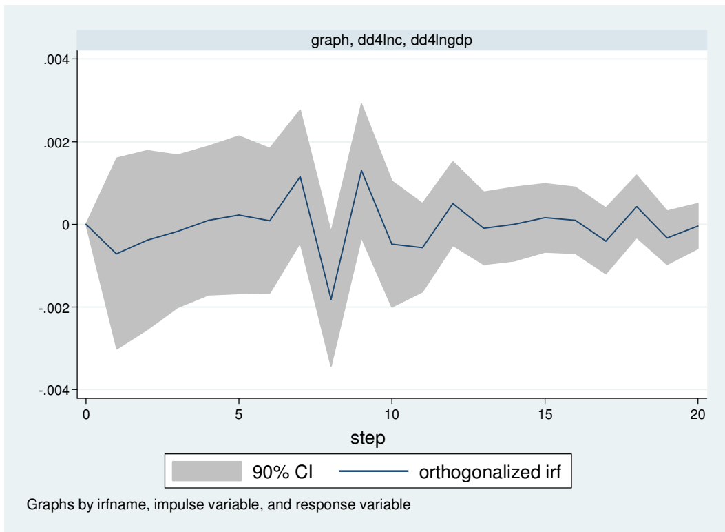
Figure 7: Orthogonalized impulse response function for an (nGDP, C) VAR model: Response of nGDP to C.
