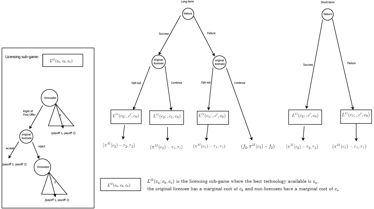
Figure 2: Period 2 Subgame Trees for Long-term and Short-term Fixed-Fee Contracts
