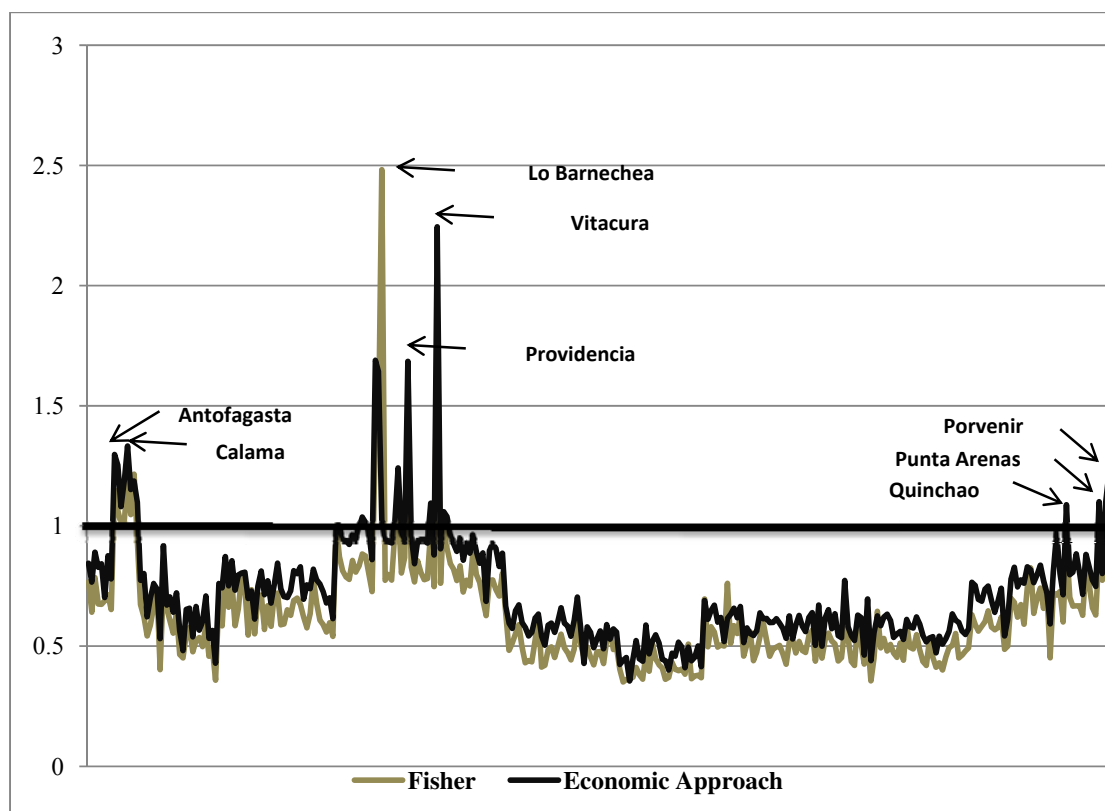
Figure 2: SHPI for Chilean communes according to the axiomatic approach versus the economic approach.
