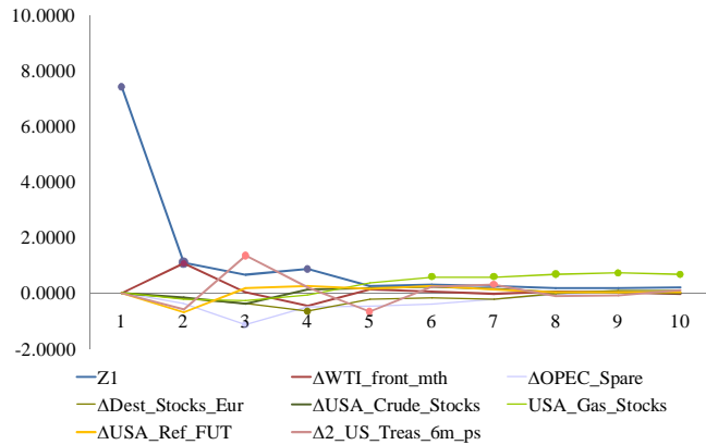
Figure A.3 - Impulse-Response for Z1 (3 lags)
