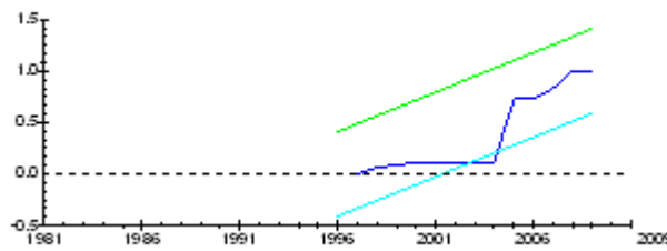
Figure 2 Cumulative Sum of Square Recursive Residual
