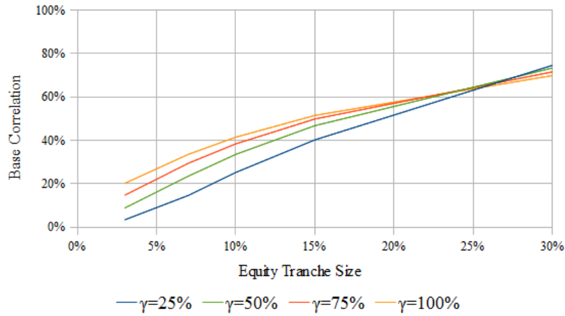
Figure 9: Base correlations for \gamma = 25\%, 50\%, 75\%, 100\% with fixed \kappa = 25\% . Recovery rate is random as in (68) with R_0 = 65\% , R_s = 25\% and R = 55\%, 45\%, 35\%, 25\% respectively given by (69). Maturity is 5 years and reference spread is at 100bp.
