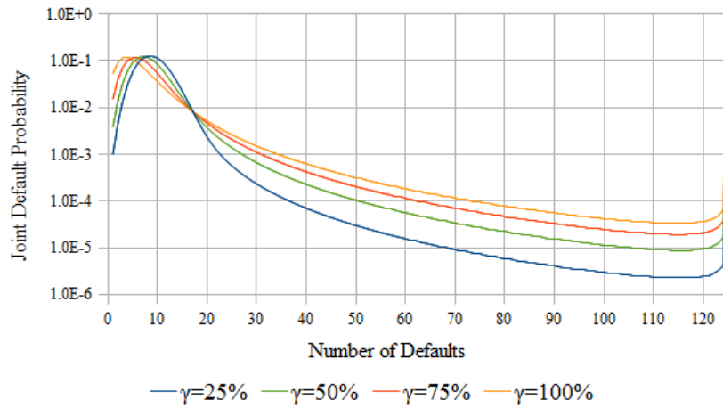
Figure 11: Joint default probability distributions for \gamma = 25\%, 50\%, 75\%, 100\% with fixed \kappa = 25\% and recovery rate R = 40\% . Maturity is 5 years and reference spread is at 100bp.
