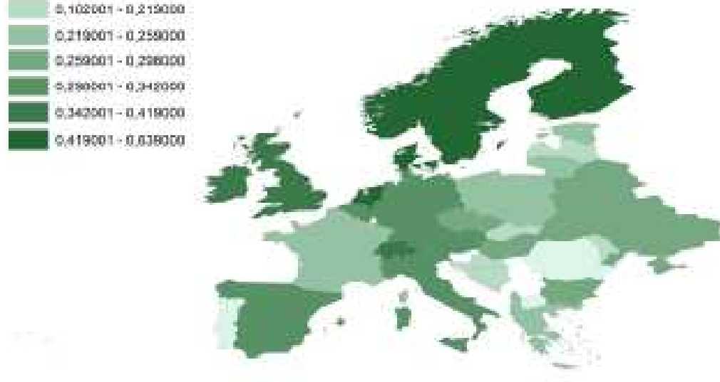
FIGURE C.2: Land Suitability and Trust-Europe
