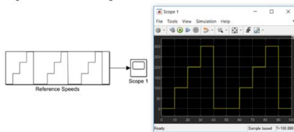
Figure 1. Reference input in the Simulink model for both Buck and Boost converters
