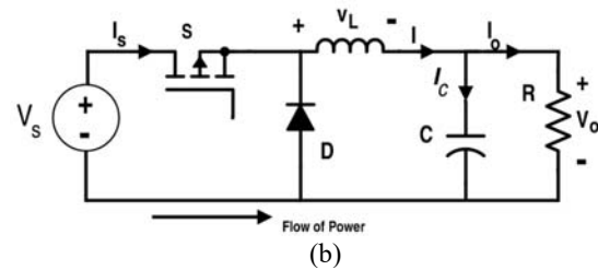
Figure 6. (a) Boost and (b) Buck converter circuit design using the GaN and SiC switches
