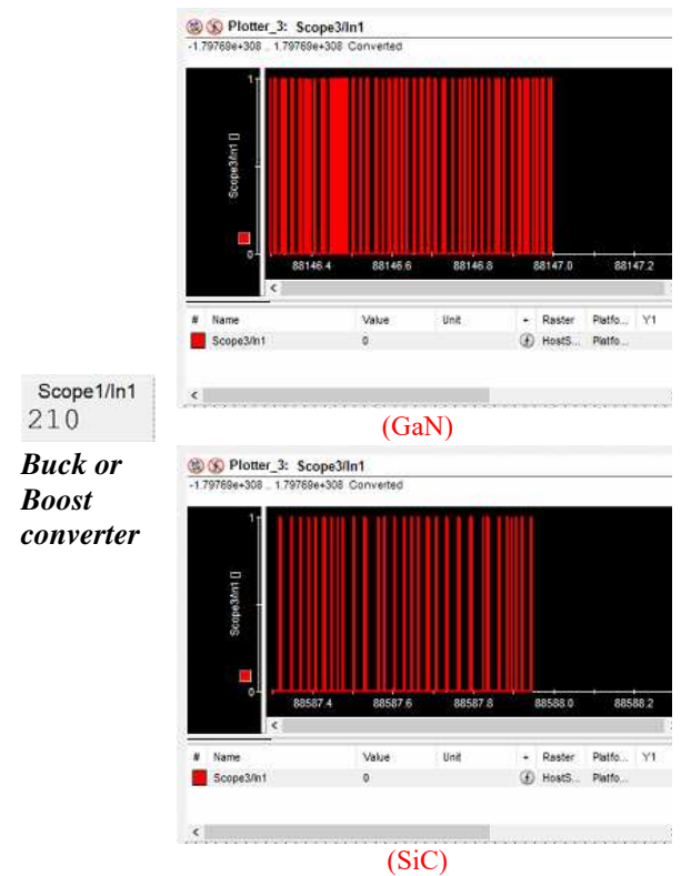
Figure 9. The output of the Hysteresis speed controller (scope 3 on dSPACE screen) in Buck or Boost converters at 210 rpm
