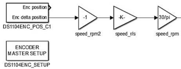
Figure 2. Calculating the speed of the motor by using gain blocks. This applies to both converters
