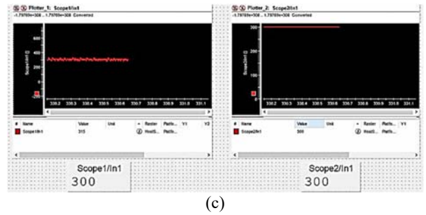
Figure 8. The output of the reference speed and dSPACE speed (scope 1 and 2 on dSPACE screen) in Buck and Boost converters at different speed (a) 100rpm, (b) 200rpm, (c) 300rpm
