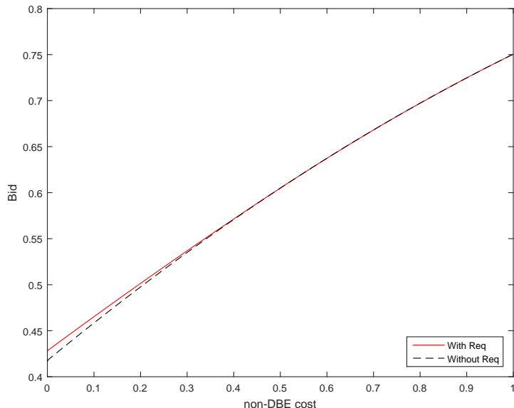
Figure 3: Bid Function
