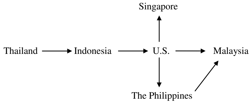
Figure 1: Short-run causality effect [pre-crisis (with U.S.)]
