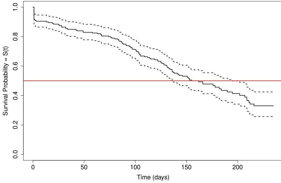
Figure 3: Kaplan-Meier. Daily new cases of COVID-19.
