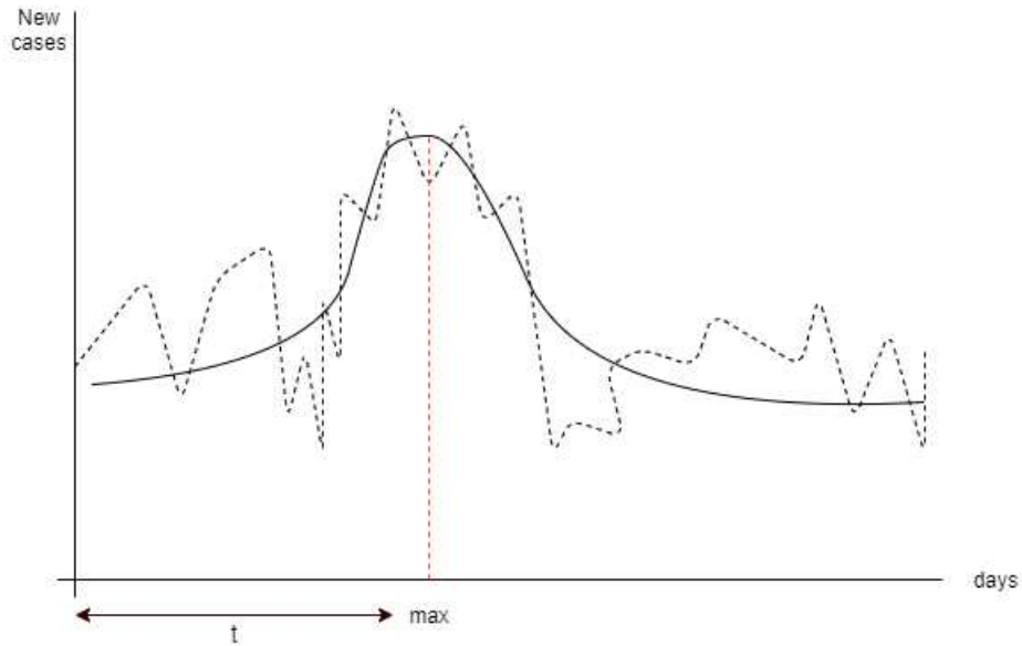
Figure 1: New cases evolution with maximum level.
