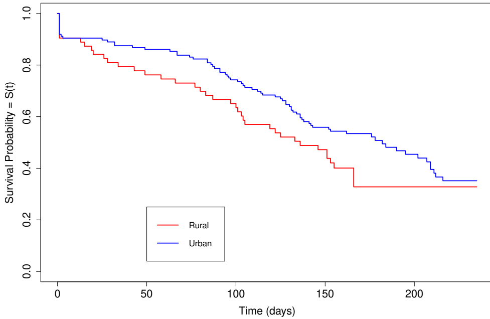
Figure 4: Kaplan-Meier. Daily new cases of COVID-19 conditioned to the level of urbanization.
