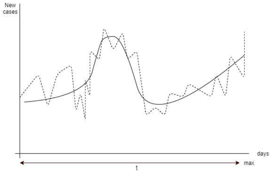
Figure 2: New cases evolution with maximum level.
