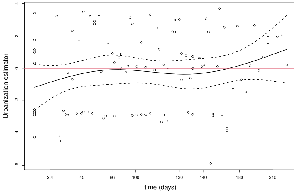
Figure 6: Linearity estimator analysis for urbanization estimator.
