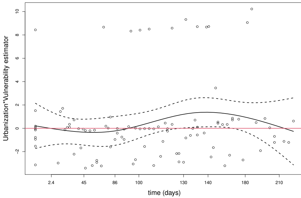
Figure 7: Linearity estimator analysis for urbanizaation*vulnerability estimator.
