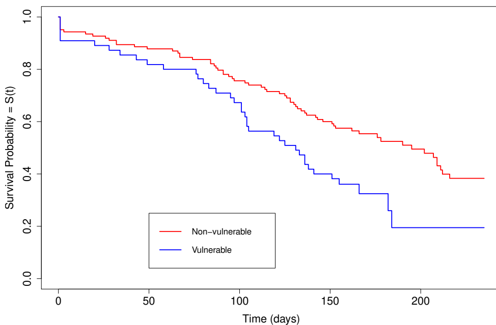
Figure 5: Kaplan-Meier. Daily new cases of COVID-19 conditioned to the level of vulnerability in the employment.
