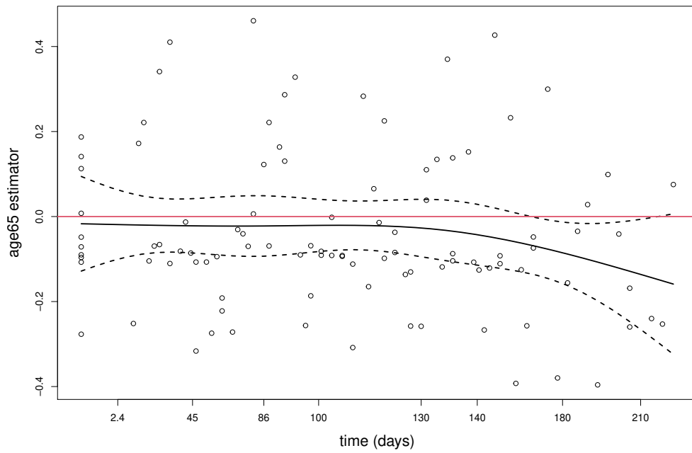
Figure 8: Linearity estimator analysis for age65 estimator.
