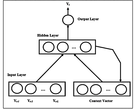
Figure 1: Elman network
