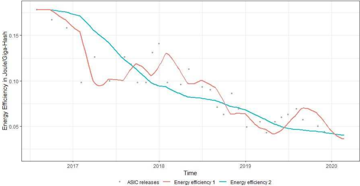
Figure 3: Energy efficiency curves estimated with models 1 and 2 in (4) for the whole Bitcoin network, and the respective ASIC releases. The reported data are measured in Joule/Giga-Hash.
