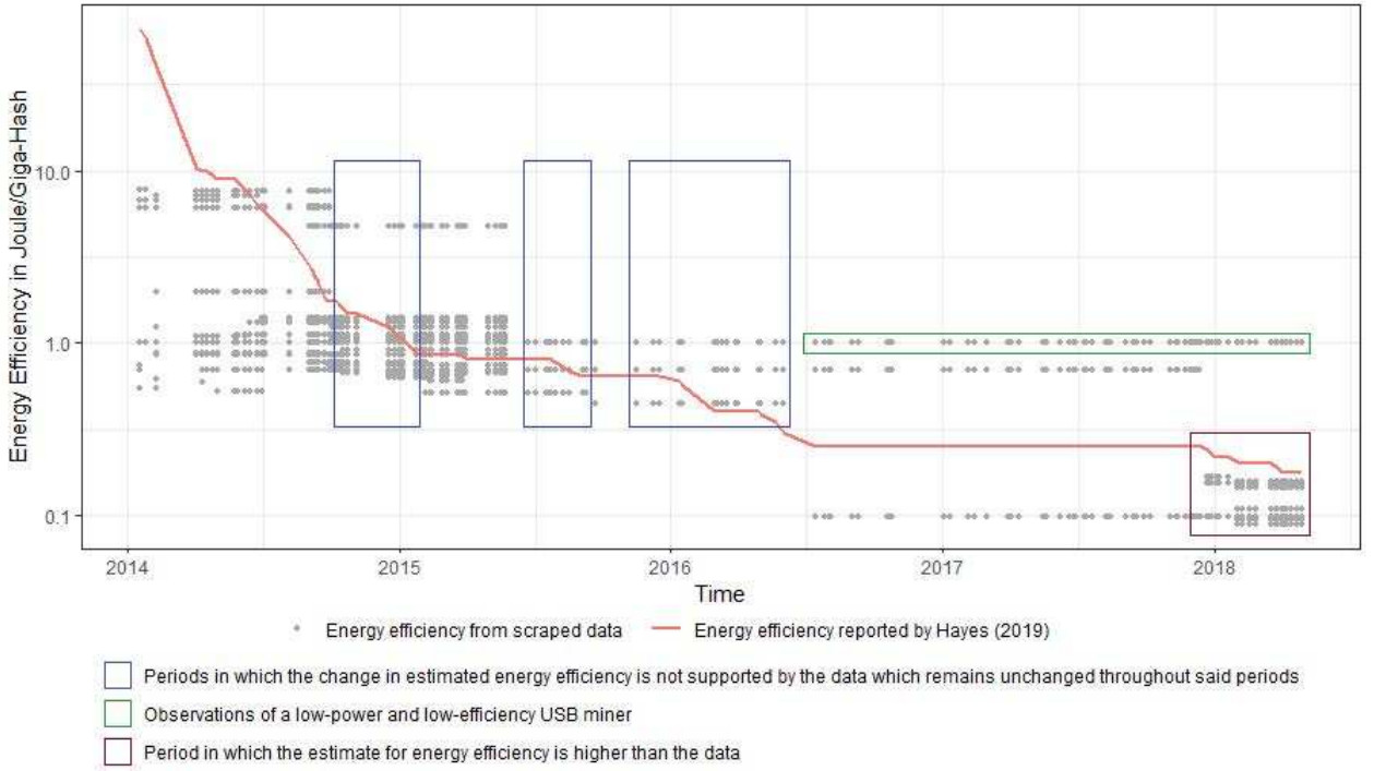
Figure 2: Energy efficiency of ASIC data scraped from the “Mining hardware comparison” webpage, and the network energy efficiency reported by Hayes (2019). Logarithmic scale.
