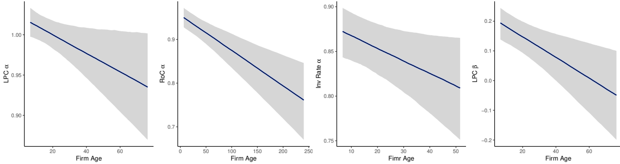
Figure 12: Marginal effects of Firm Age on \alpha of labor productivity change ( \Delta LP ), profitability ( ROC ), and investment rate IR , and \beta of \Delta LP . The blue line is the mean estimate and the grey shade area is the 90% uncertainty interval.
