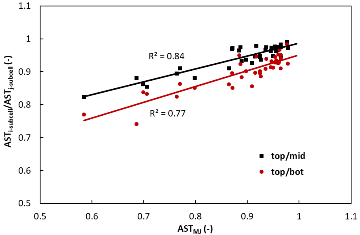
Figure 5. Ratio of the AST for the i -subcell ( AST_{i\text{-subcell}} ) to the AST for the j -subcell ( AST_{j\text{-subcell}} ) versus the AST of soiling across the spectral region of the multi-junction (MJ) solar cell considered.
