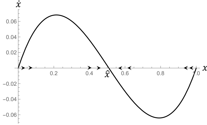
Fig. 1 Steady states without the state of emergency
