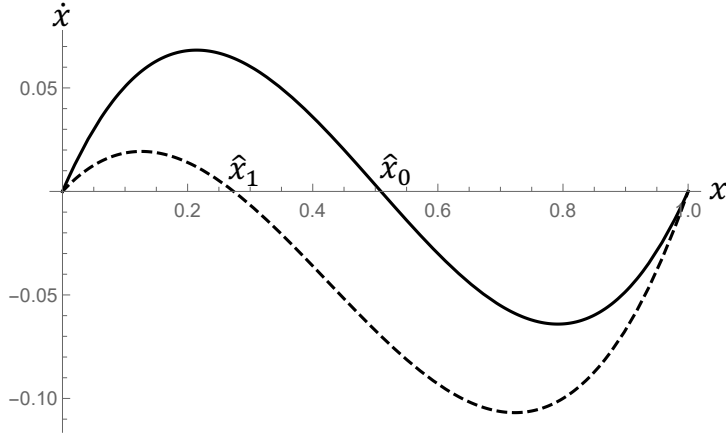
Fig. 2 Effect of the state of emergency
