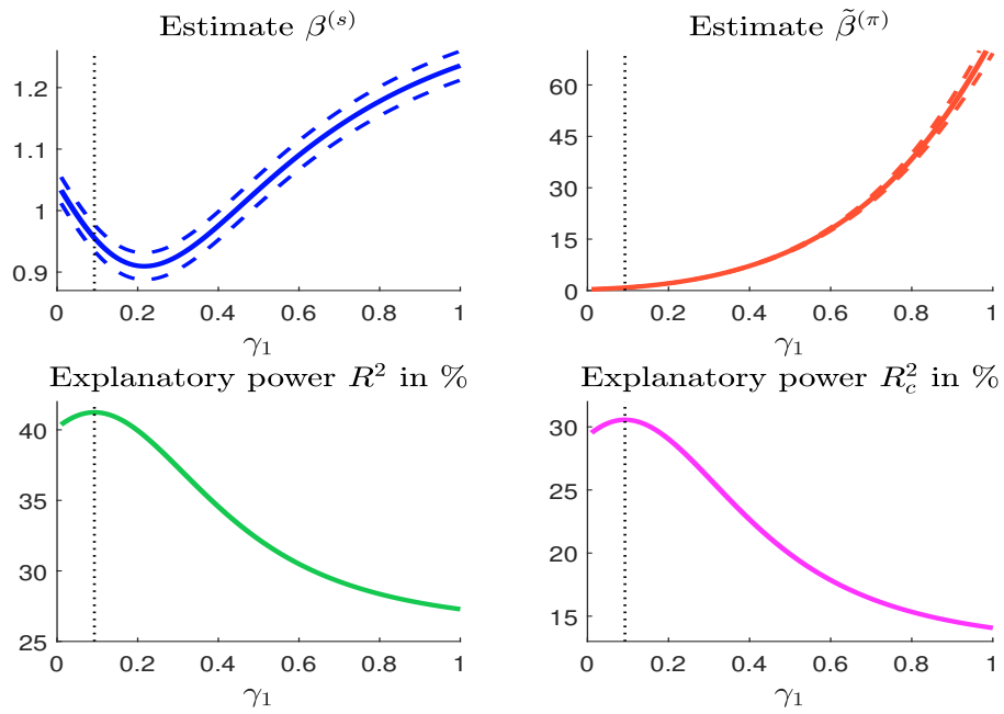
Figure 22: Parameter estimation using the grid-search approach
