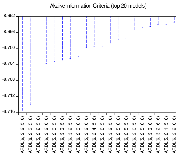
Figure 1. Akaike Info Criterion
