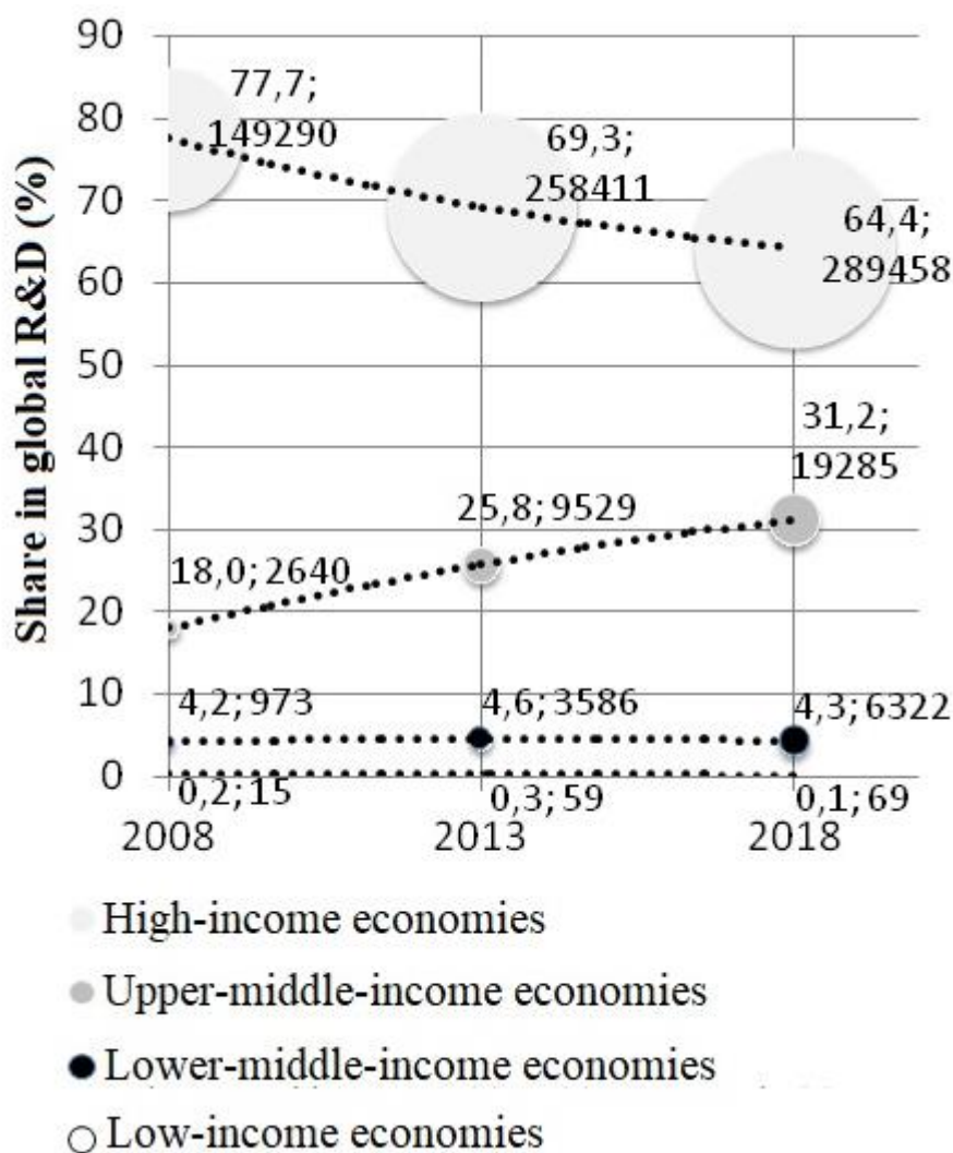
Figure-2. Changes in global indicators. Data signatures: «Share in global R&D» and «Number of granted patents (USPTO)» (bubble size). The source: UNESCO Science Report (2016, 2021).
