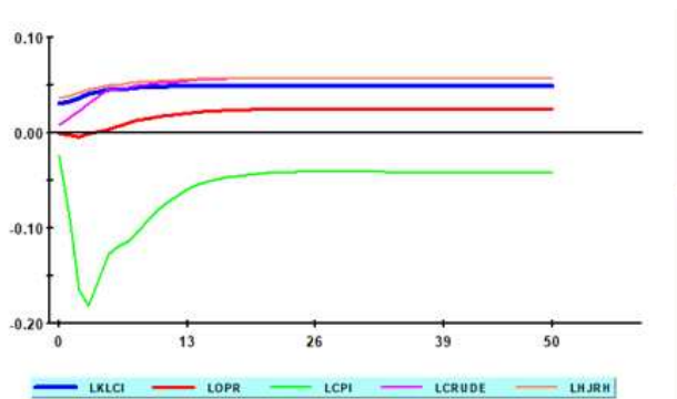
Figure 4 Generalized Impulse Response to stock to each variable
