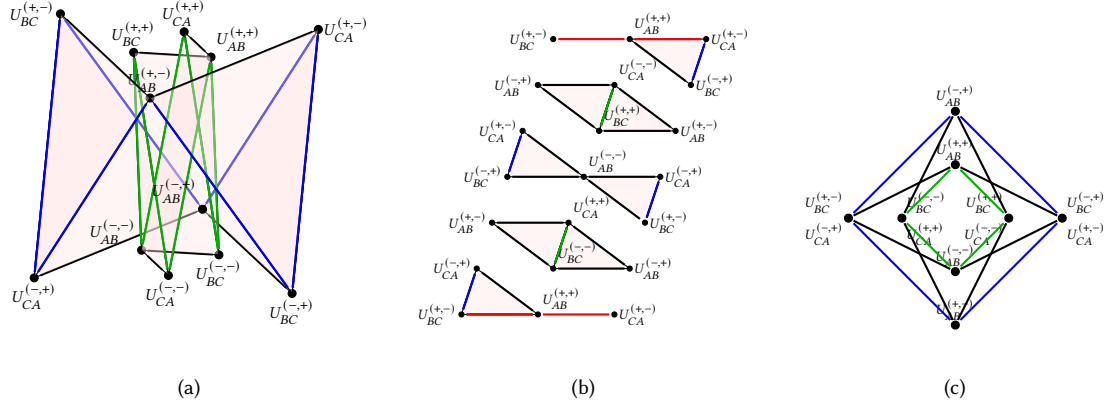
Fig. 10. The restricted domain N''_I is the union of the simplicial complexes represented in (a) and (b) according the identifications defined by vertices' labeling and colours. The simplicial complex N^* is represented in (c). The colours of the edges (resp. the labelings of the vertices) show where the edges (resp. the vertices) of N''_I have been compressed in N^* .
