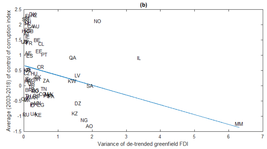
Figure 1: Relationship between variance of greenfield FDI and information frictions
