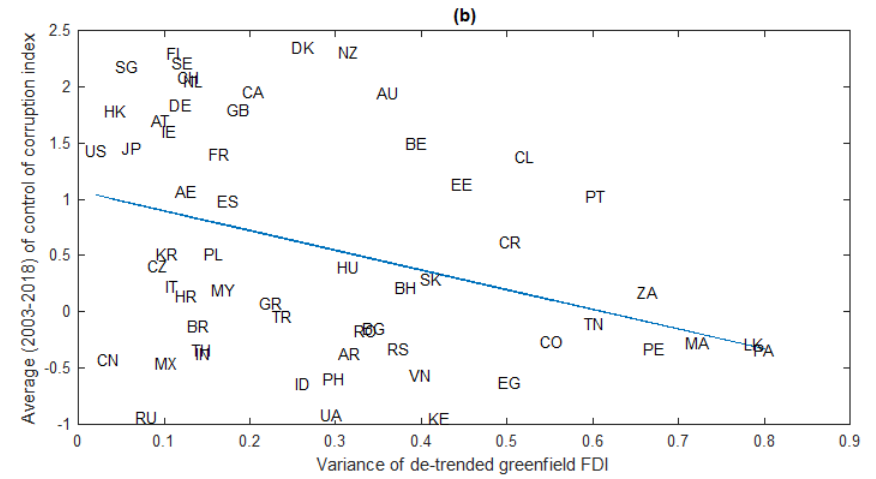
Figure A1: Relationship between variance of greenfield FDI and information frictions, economies with a variance of less than one
