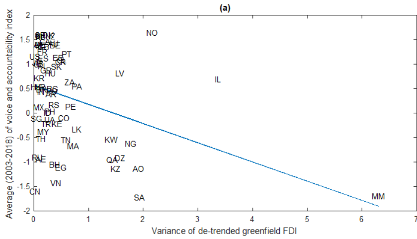
Figure 1: Relationship between variance of greenfield FDI and information frictions
