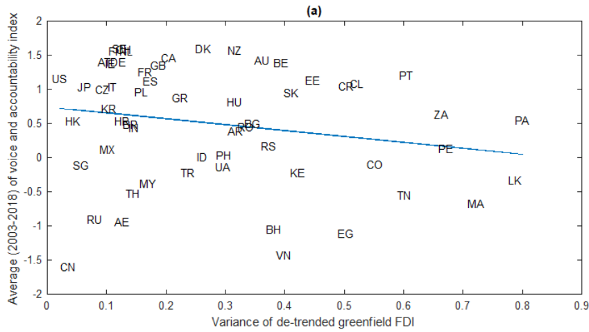
Figure A1: Relationship between variance of greenfield FDI and information frictions, economies with a variance of less than one
