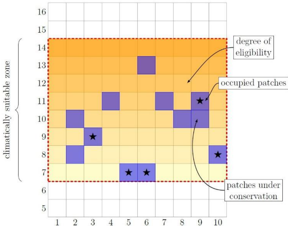
Figure A5: 'Climate change directional prioritization strategy'. The red-framed area represents the climatically suitable zone (CSZ), within which the orange-shaded area represents patches eligible for patch selection in the 'climate change directional prioritization strategy'. The degree of orange depicts the level of eligibility of a particular patch; darker-shaded areas have a higher eligibility than lighter-shaded areas. The blue shaded area represents a patch selected for conservation; the star-symbol indicates that this patch is occupied by the target species.
