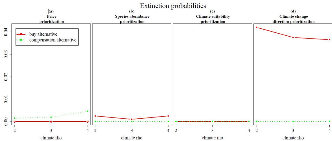
Figure A13: Extinction probabilities of the different GM-PSS pairs with changing climate suitability bell curvature parameter \rho . The red line represents results for the buy alternative, the green line for the compensation alternative.
