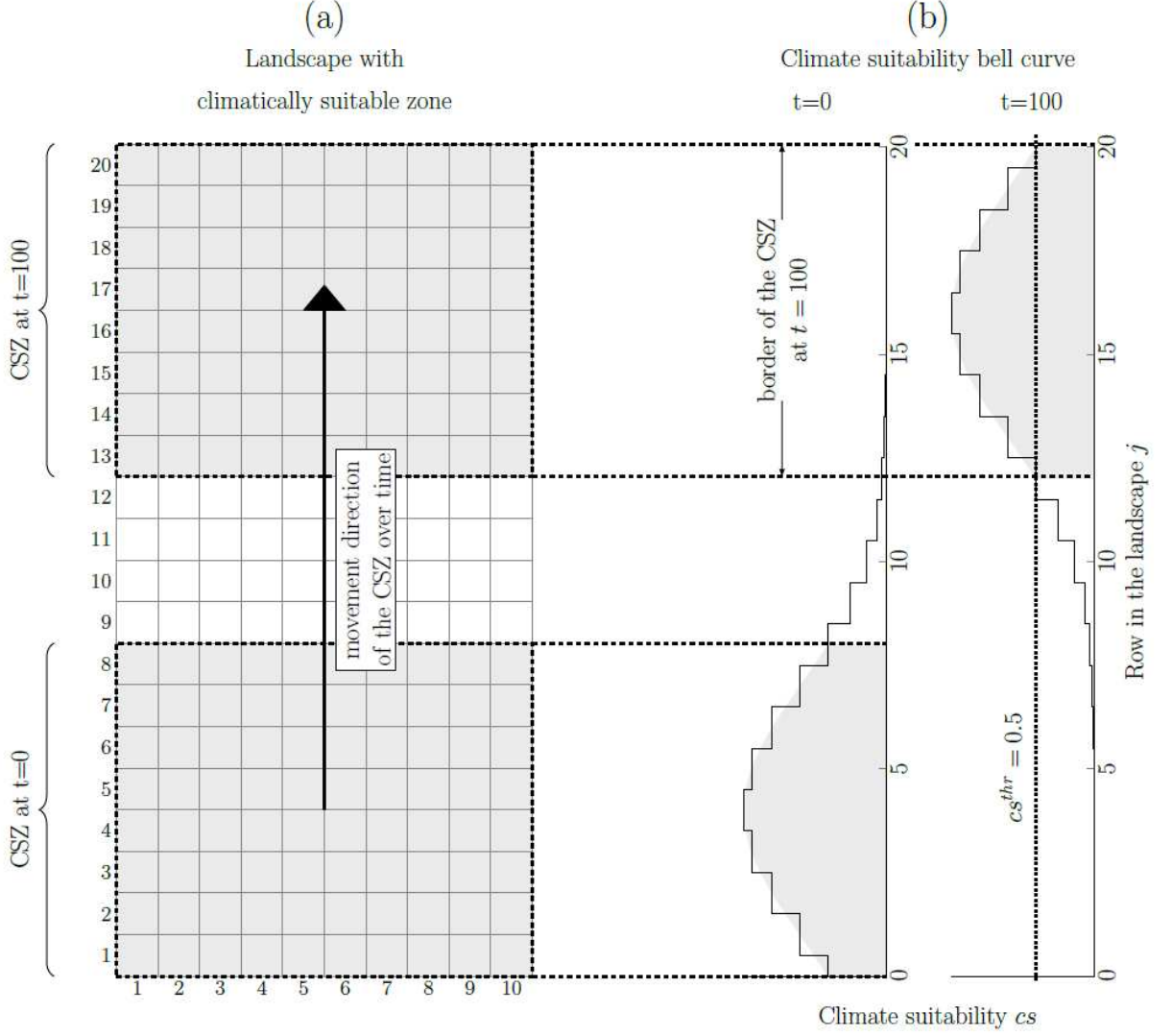
Figure 1: (a) Spatially explicit landscape consisting of 10 \times 20 patches including the climatically suitable zone (CSZ, shaded area) at time-steps t = 0 and t = 100 , (b) climate suitability bell curves according to Eq. (1) in their respective base case parametrization (see Table 2) and climate suitability threshold cs_{thr} = 0.5 , leading to the CSZ at the different time steps t \in \{0, 100\} . The shaded area and the corresponding borders represent the CSZ at time-steps t = 0 and t = 100 .
