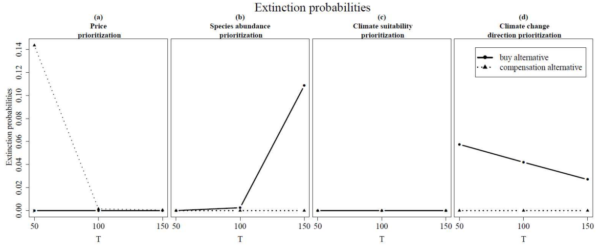
Figure 3: Changes in extinction rates due to changes in maximum length of the simulation timeframe T , (i.e. climate change speed decreases with increasing T ). (a)-(d) represent the extinction probabilities for all four strategies in the buy and compensation alternative.
