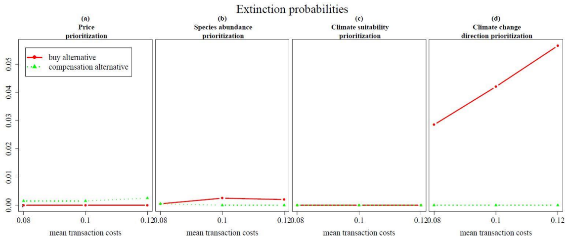
Figure A11: Extinction probabilities of the different GM-PSS pairs with changing mean transaction costs. The red line represents results for the buy alternative, the green line for the compensation alternative.
