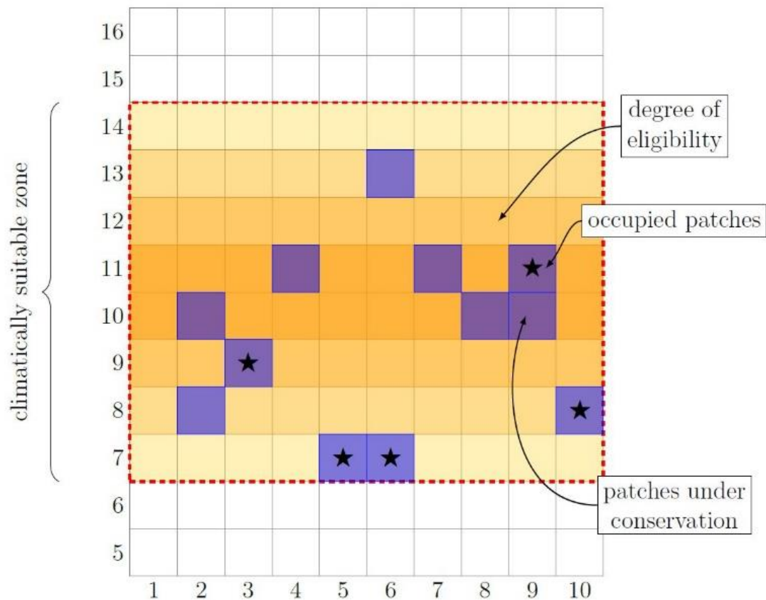
Figure A4: ‘Climate suitability prioritization strategy’. The red-framed area represents the climatically suitable zone (CSZ), within which the orange-shaded area represents patches eligible for patch selection in the ‘climate suitability prioritization strategy’. The degree of orange depicts the level of eligibility of a particular patch; darker-shaded areas have a higher eligibility than lighter-shaded areas. The blue shaded area represents a patch selected for conservation; the star-symbol indicates that this patch is occupied by the target species.
