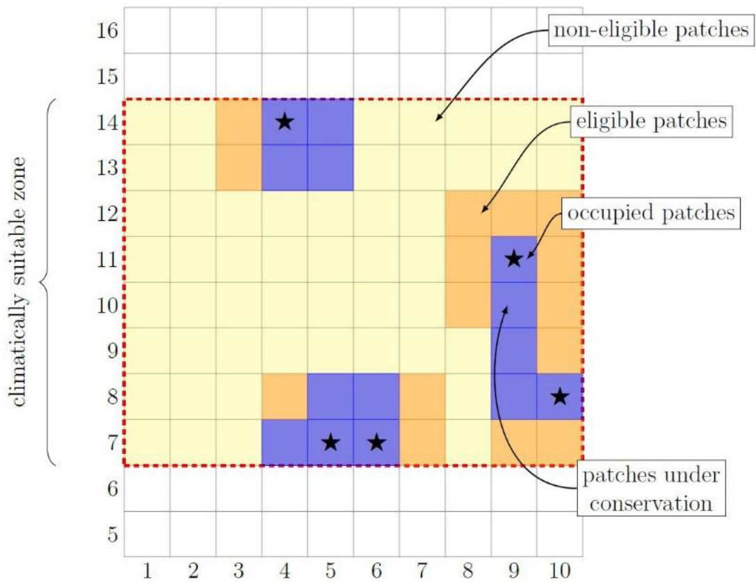
Figure A3: ‘Species abundance targeting strategy’. The red-framed area represents the climatically suitable zone (CSZ), within which the orange-shaded area represents patches eligible for patch selection in the ‘species abundance targeting strategy’. The yellow-shaded areas represent patches, which are non-eligible for selection in this strategy. The blue shaded area represents a patch selected for conservation; the star-symbol indicates that this patch is occupied by the target species.
