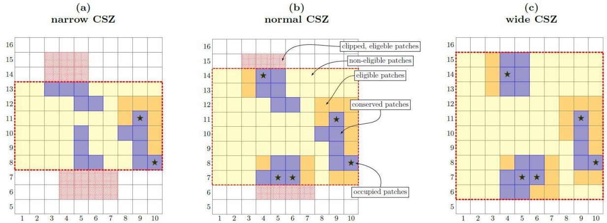
Figure A6: Patch restriction effect in the ‘species abundance prioritization strategy’ due to changes in CSZ sizes due to varying cs^{thr} . The red-framed area represents the climatically suitable zone (CSZ), within which the orange-shaded area represents patches eligible for patch selection in the ‘species abundance prioritization strategy’. The degree of orange depicts the level of eligibility of a particular patch; darker-shaded areas have a higher eligibility than lighter-shaded areas. The blue shaded area represents a patch selected for conservation; the star-symbol indicates that this patch is occupied by the target species. The red-shaded areas represent patches which could have been selected by the respective strategy, if the CSZ was large enough, but in fact are restricted in eligibility by the patch restriction effect.
