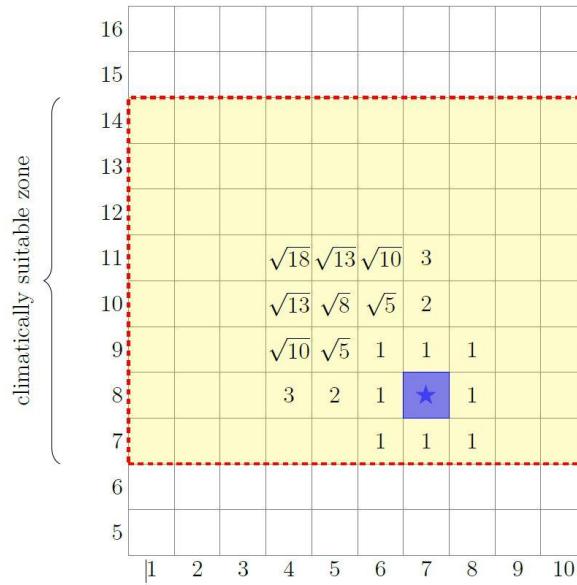
Figure F1: Distance between two patches calculated by Eq. (A1). The yellow-shaded and red-framed area represents the climatically suitable zone (CSZ). The blue-shaded area represents a patch selected for conservation; the star-symbol indicates that this patch is occupied by the target species. Numbers indicate the distance of the respective patch to the highlighted blue patch. Note that the distance for all patches directly neighbouring the blue patch is 1.
