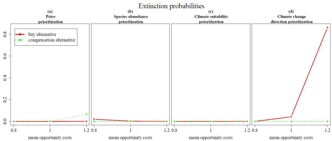
Figure A8: Extinction probabilities of the different GM-PSS pairs with changing mean opportunity costs. The red line represents results for the buy alternative, the green line for the compensation alternative.
