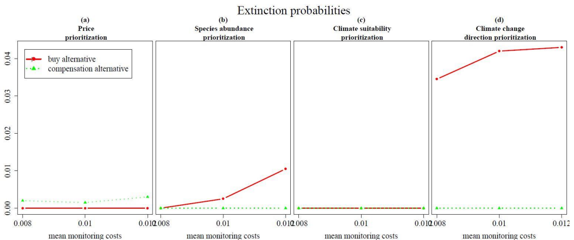
Figure A12: Extinction probabilities of the different GM-PSS pairs with changing mean monitoring costs. The red line represents results for the buy alternative, the green line for the compensation alternative.
