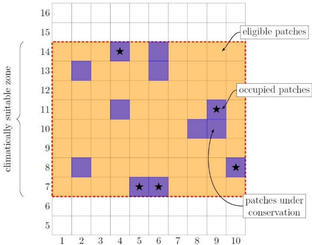
Figure A2: 'Prize prioritization strategy'. The red-framed area represents the climatically suitable zone (CSZ), within which the orange-shaded area represents patches eligible for patch selection in the 'prize prioritization strategy'. The blue-shaded area represents a patch selected for conservation; the star-symbol indicates that this patch is occupied by the target species.
