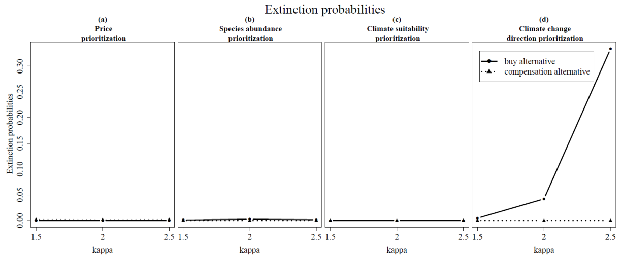
Figure 5: Influence of changes in \kappa on the extinction probability in the buy alternative and the compensation alternative for each of the four PSSs.
