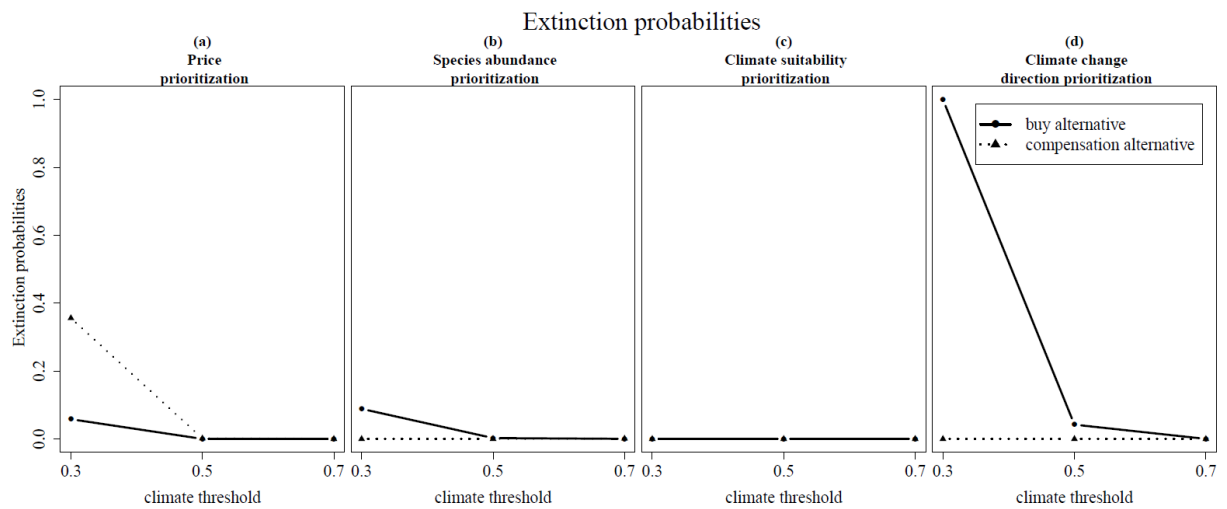
Figure 4: Extinction probabilities of the different GM-PSS pairs with changing climate threshold, resulting in changing CSZ sizes.
