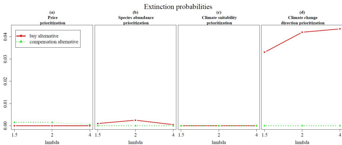
Figure A14: Extinction probabilities of the different GM-PSS pairs with changing climate direction prioritization strength \lambda . The red line represents results for the buy alternative, the green line for the compensation alternative.
