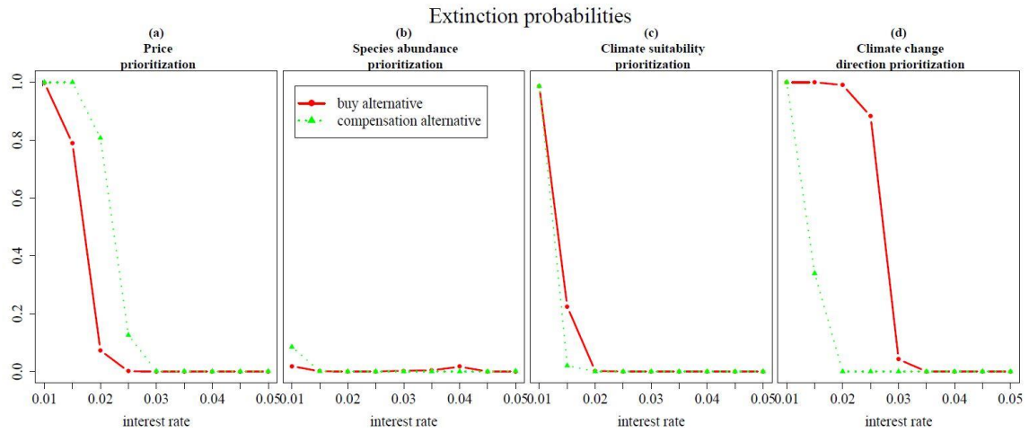
Figure A7: Extinction probabilities of the different GM-PSS pairs with changing interest rates, resulting in changes in available budgets and discount rates. The red line represents results for the buy alternative, the green line for the compensation alternative.
