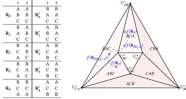
Fig. 11. On the left side, the sequences R and R' are defined. Writing an alternative on the top on another means that the one on top is preferred to the one in the bottom. On the right side there is a graphical representation of the paths defined by f(R) .
