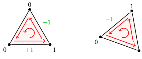
Fig. 15. On the left, the contribution of the simplex is 0 because the two edges \vec{01} compensate each other. On the right, the contribution of the tricoloured triangle is -1 .
