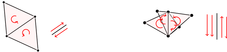
Fig. 14. The simplicial complex on the left is oriented because the induced orientations on the inner edge are opposite. However, the right one is not because it has three orientations in one direction and one on the opposite direction.
