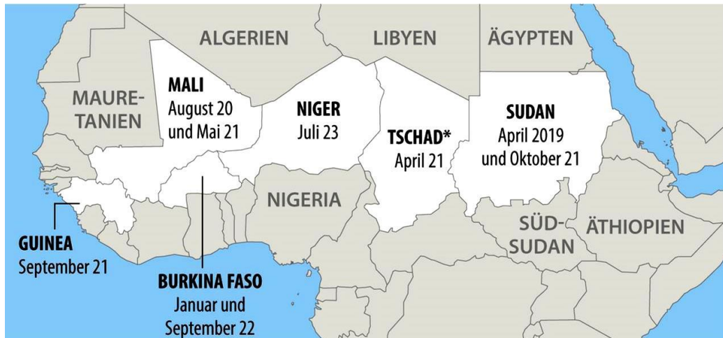
Graph 3: Military coups in the Sahel zone and West Africa since 2019
