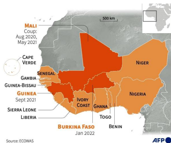
Graph 2: Map of 3 ECOWAS states suspended and sanctions imposed as of 2021
