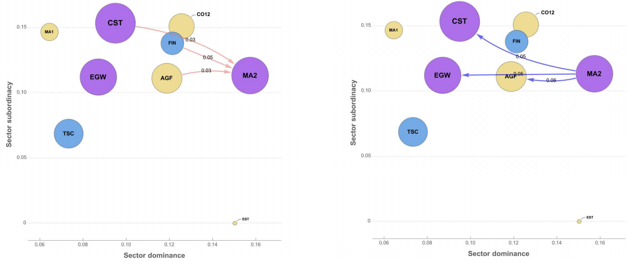
Bubble Properties: (1) Position: Coordinates of dominance (row-wise sum) and subordinacy (column-wise sum of multipliers); (2) Shape: Size of eigenvector centrality score; (3) Color: Communities of sectors; (4) Arrows: In-degree (red) or Out-degree (blue) edges with edge weights.
