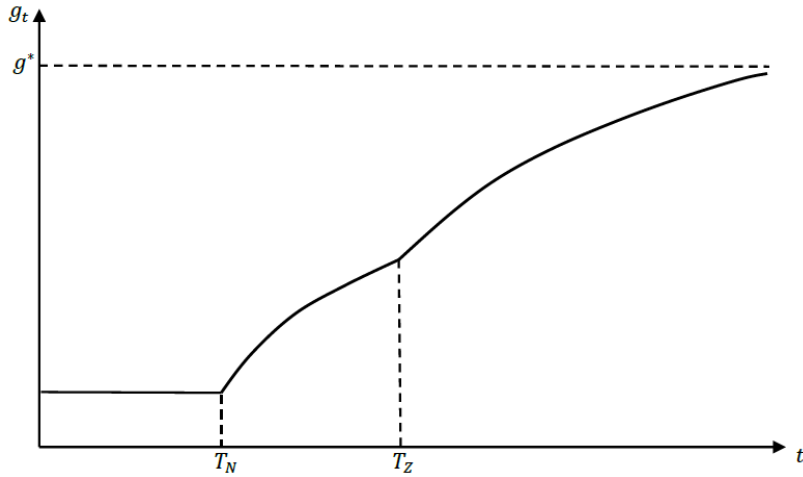
Figure 2: Transition path of the growth rate
