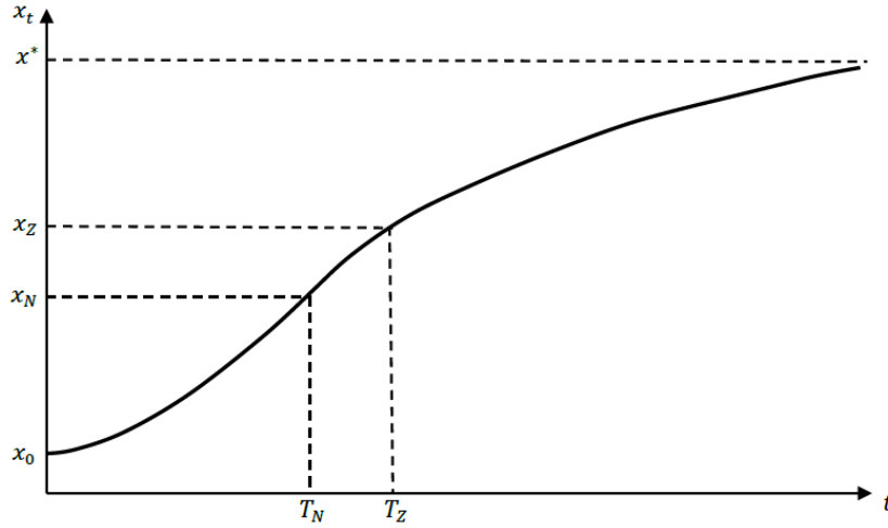
Figure 1: Transition path of the firm size
