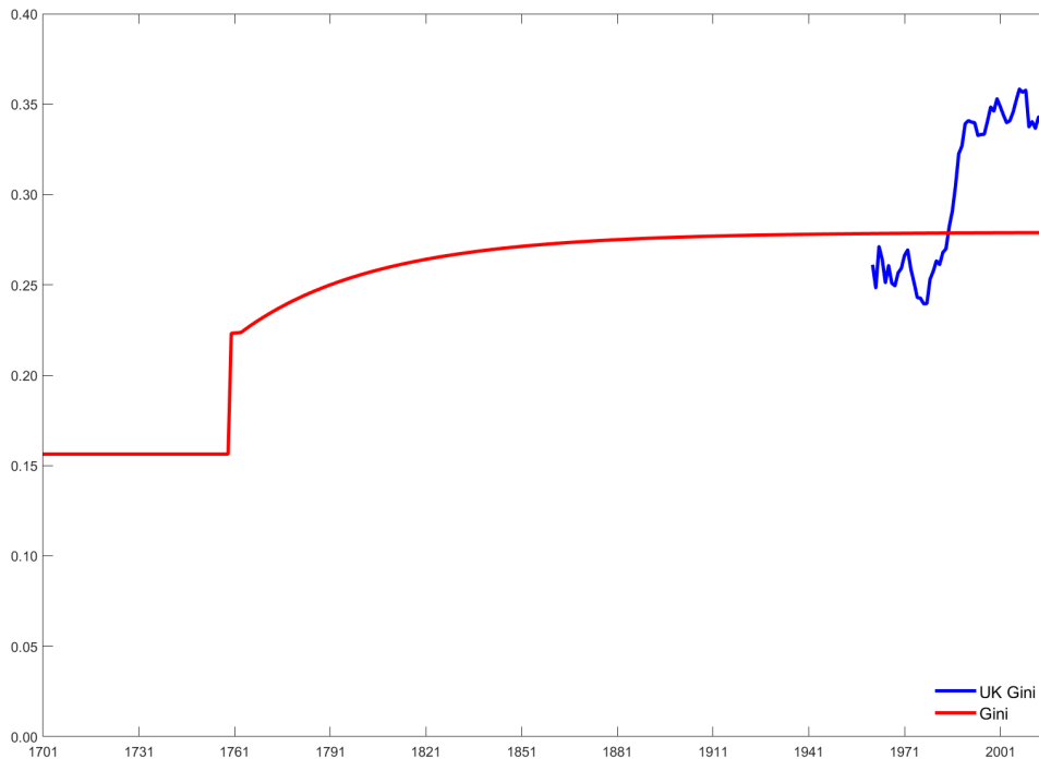
Figure 7: Simulated path of income inequality (Gini coefficient)
