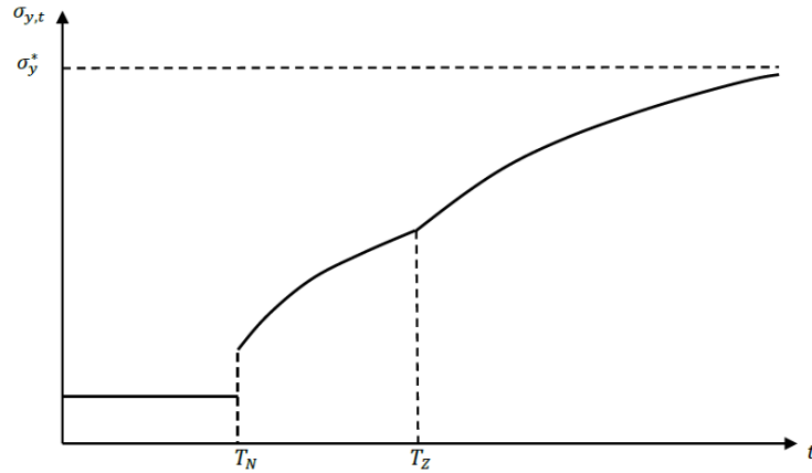
Figure 4: Transition path of income inequality
