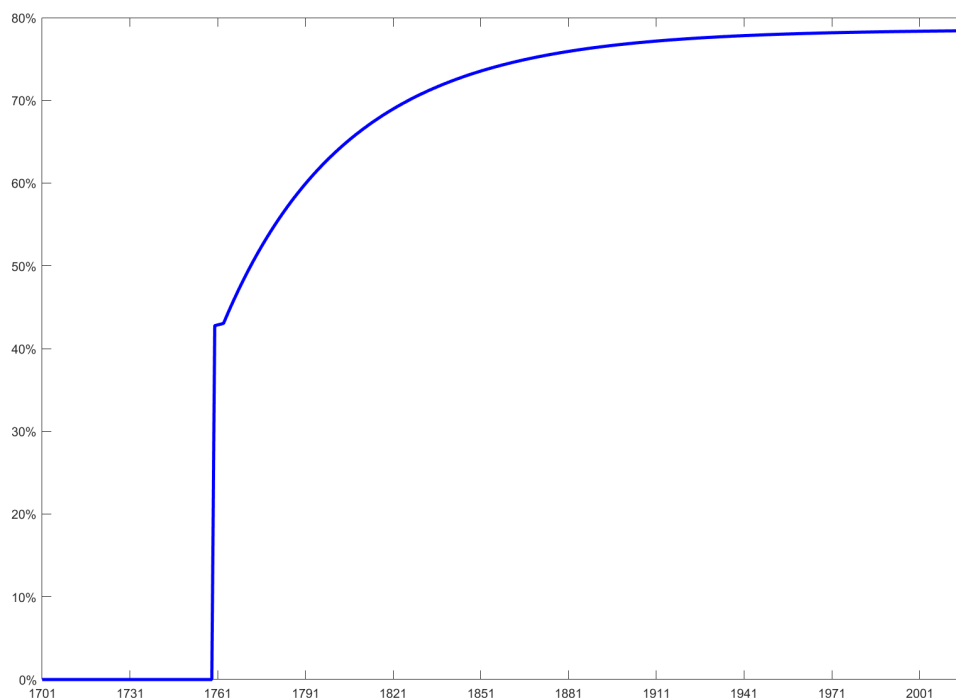
Figure 6: Simulated path of income inequality (percent change)
