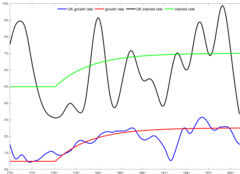
Figure 5: Simulated paths of the growth rate and the interest rate
