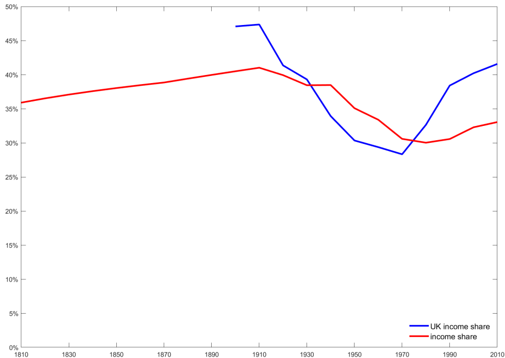
Figure 8: Simulated path of the top 10% income share
