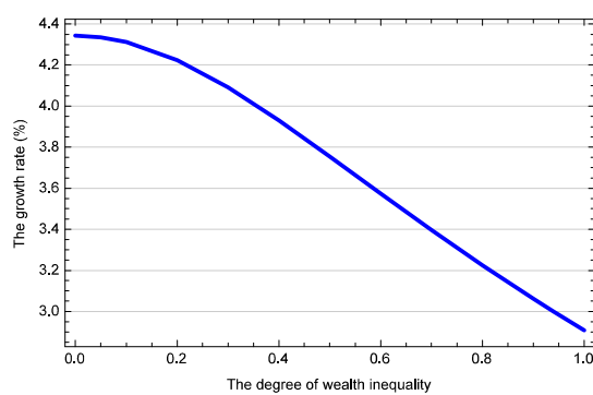
Figure 4b: Growth and inequality ( \sigma = 10 )
