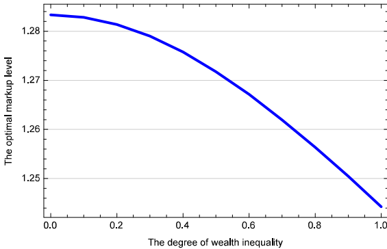
Figure 6a: Markup and inequality ( \alpha = 0.616 )
