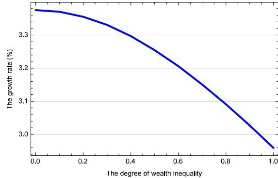
Figure 6b: Growth and inequality ( \alpha = 0.616 )
