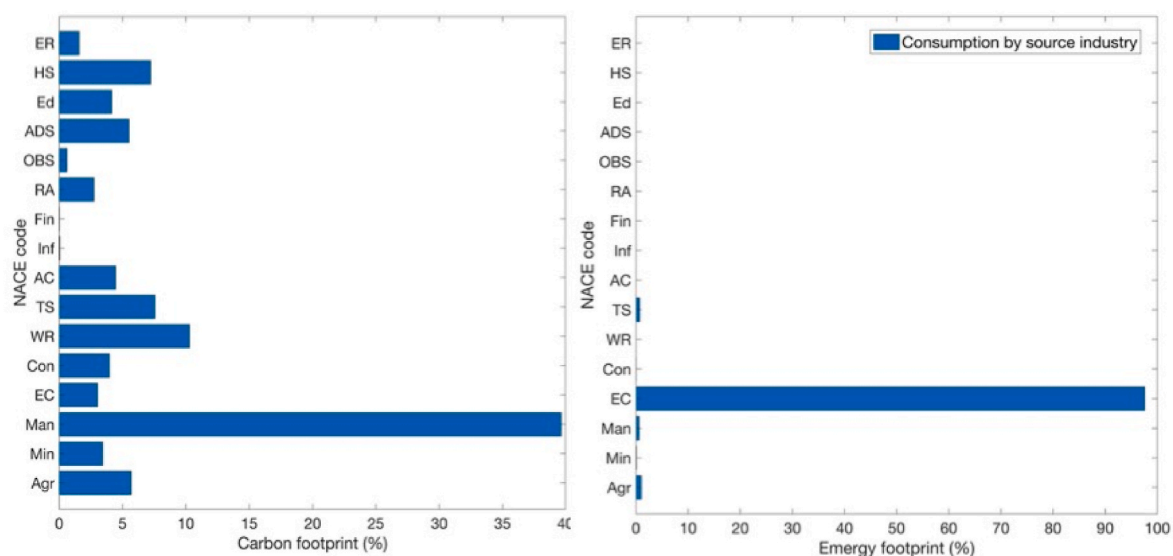
Fig. 6. Differences between the supply-extended and the use-extended model-based carbon footprint (left) and emery footprint for source sectors (right), estimated from a commodity-by-commodity IO model for Vienna 2015. The complete carbon footprint and emery-based carbon footprint details are found in the supporting information “S2 in Table S-A and S-B, respectively. Product categories follow CPA classification. Names, abbreviations of products are presented in Tables S-C in the supporting information.
