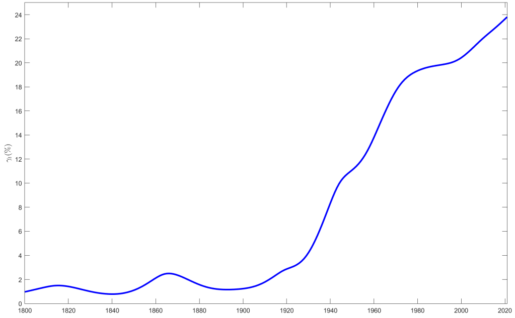
Figure 3: Trend of the US productive government spending share of GDP
