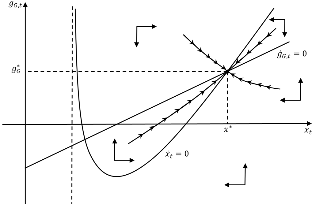
Figure D1: Phase Diagram
