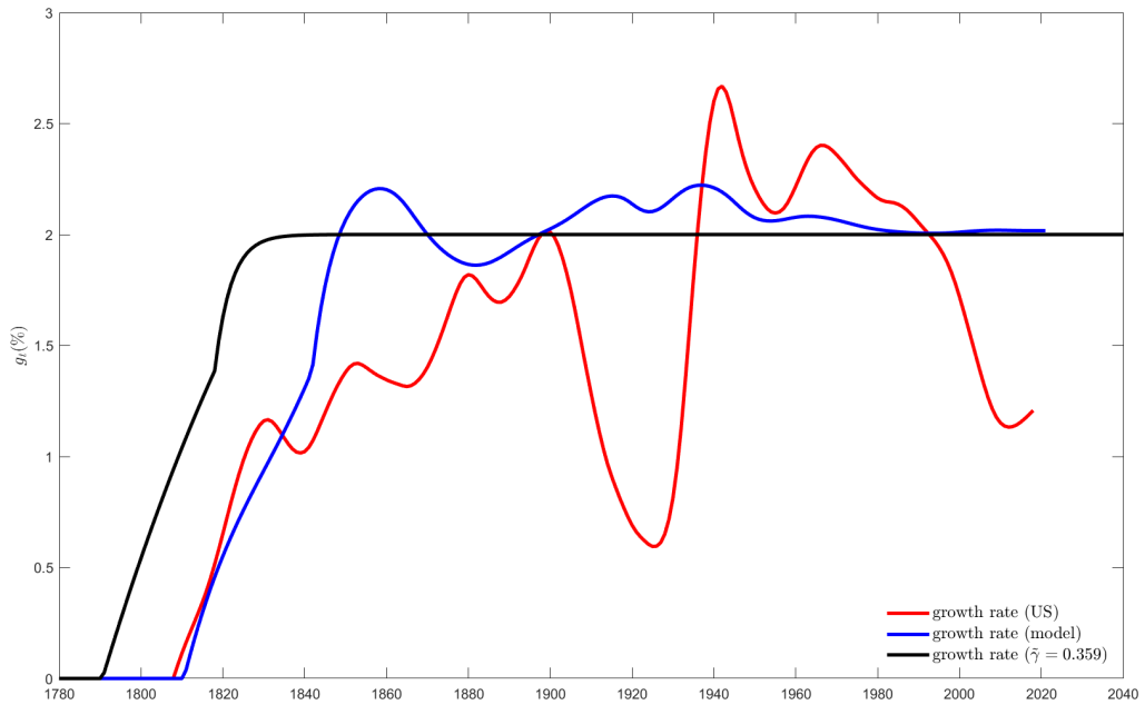
Figure 4: Effects of productive government spending ( \kappa = 0.1 )
