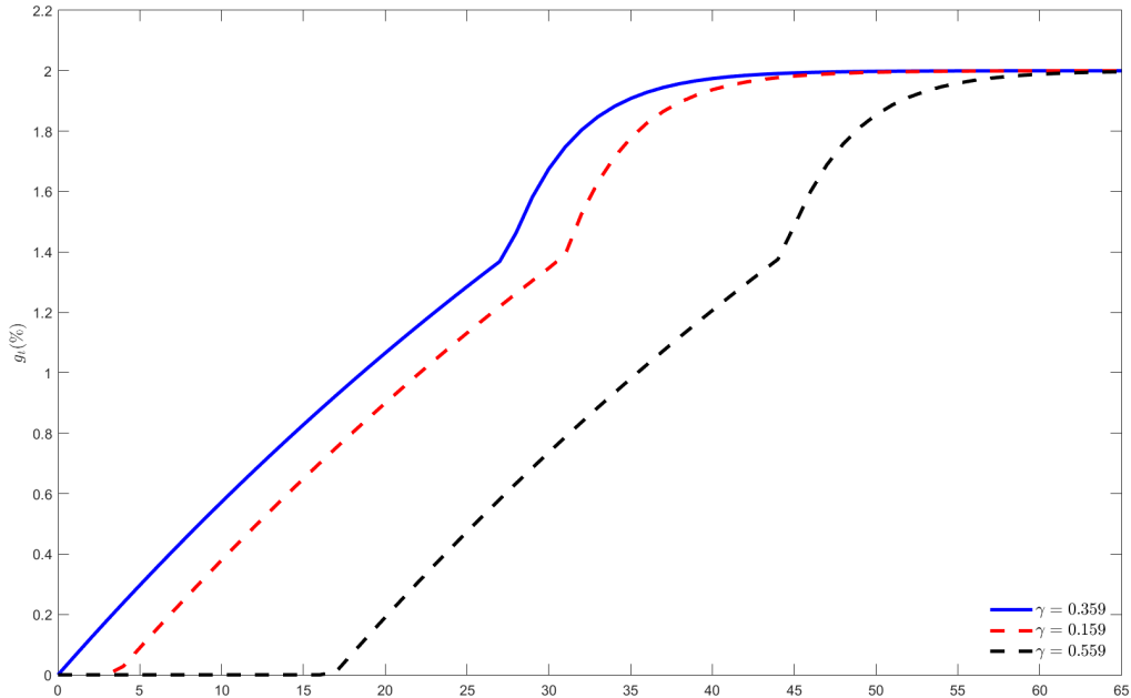
Figure 2: Deviating from the growth-maximizing value \tilde{\gamma}
