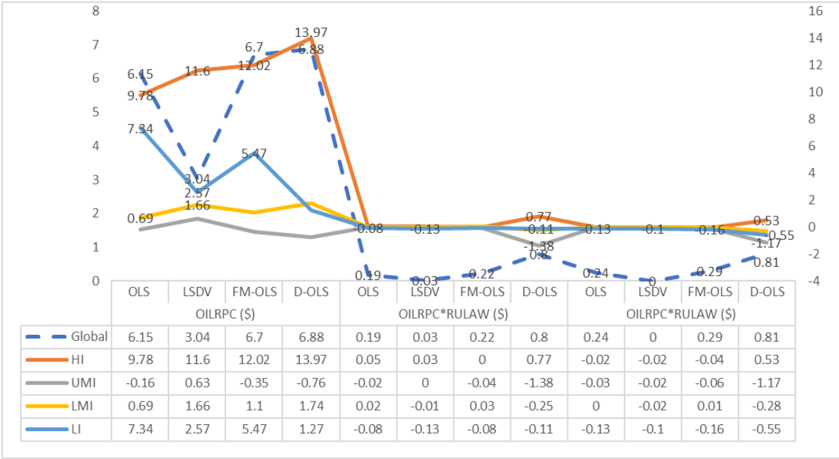
Figure 9 Impact of oil rent and its interaction with institutional variables on GDP per capita - Full (for recall) and sub-samples
