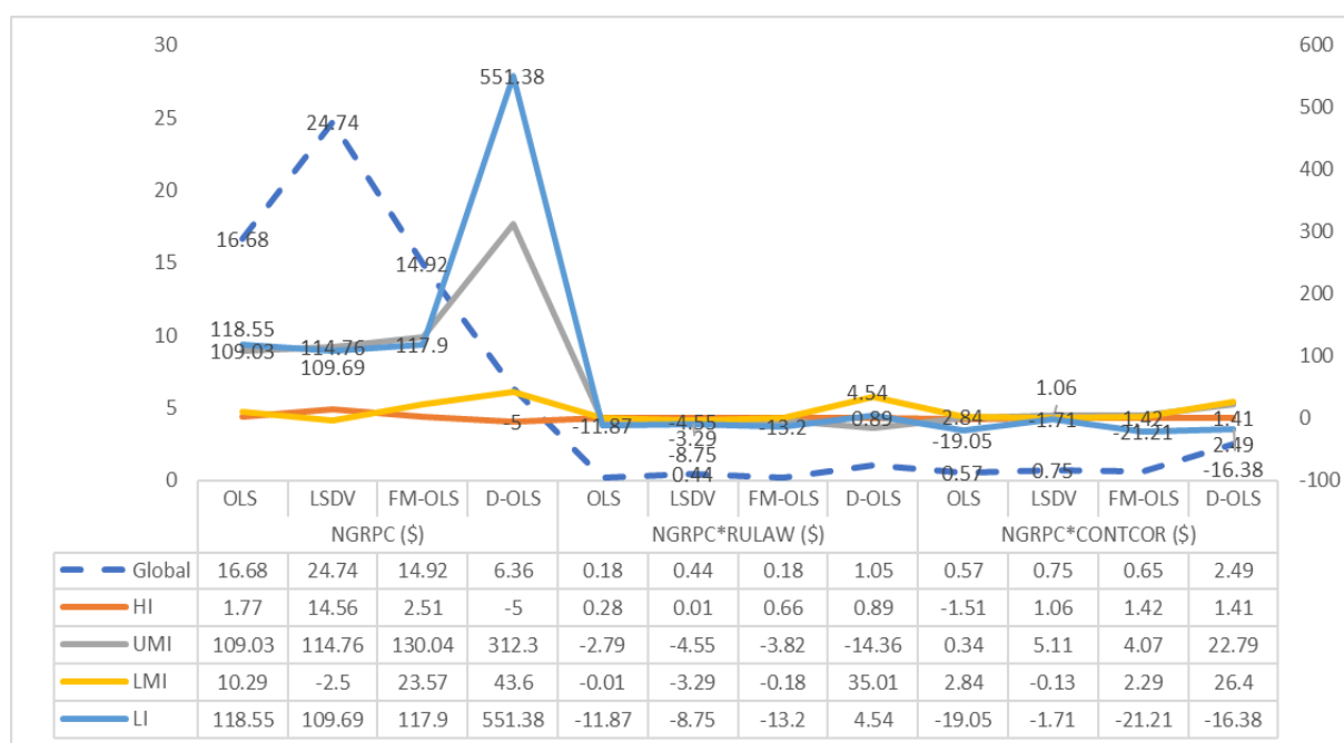
817 Figure 8 Impact of gas rent and its interaction with institutional variables on GDP per capita — Full (for recall) and sub-samples
