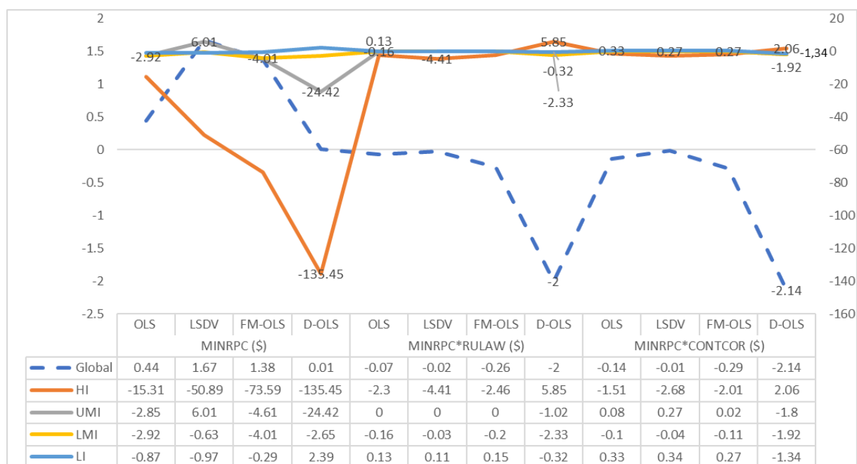
814 Figure 7 Impact of mining rent and its interaction with institutional variables on GDP per capita — Full (for recall) and sub-samples
