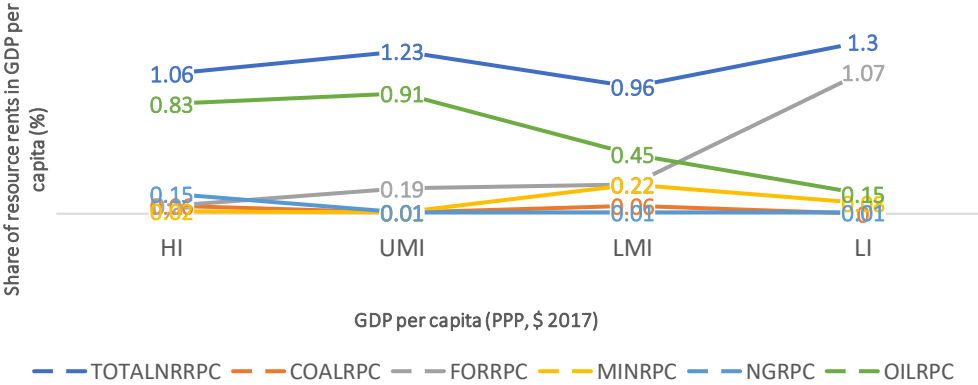
Figure 1 Relationship between the share of rents in GDP per capita and the level of GDP per capita for total resources and each of their 5 components
