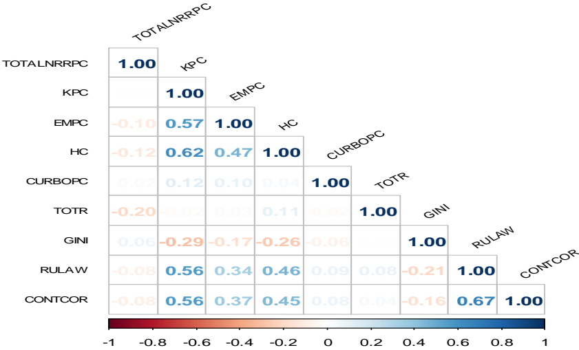
Figure 3 Correlation matrix between model explanatory variables
