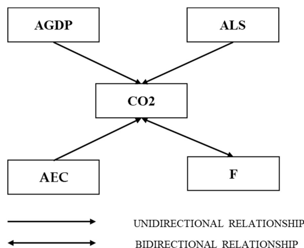
Fig. 1. Relationships between study variables established by the causality test
