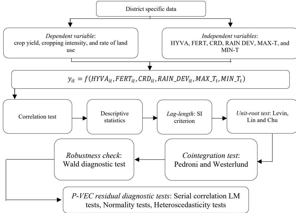
Figure 2. Flowchart illustrating data diagnosis
