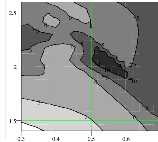
\alpha, cK, rYTFP\_PPP
