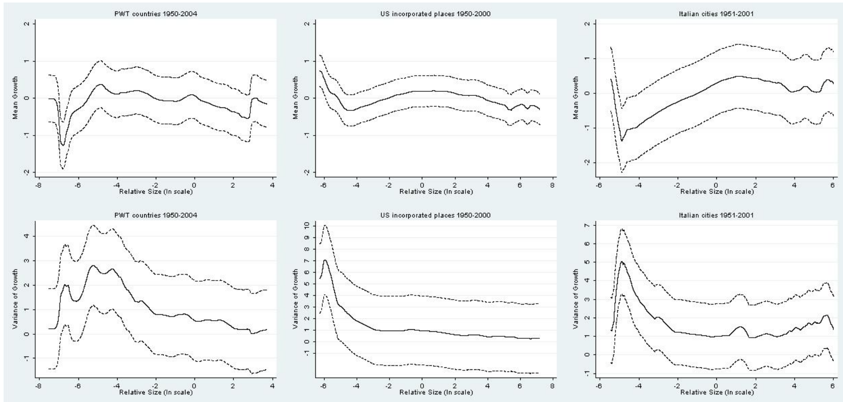
Figure 1: Estimated mean and variance of the standardized population growth in terms of relative size using kernel regression.
