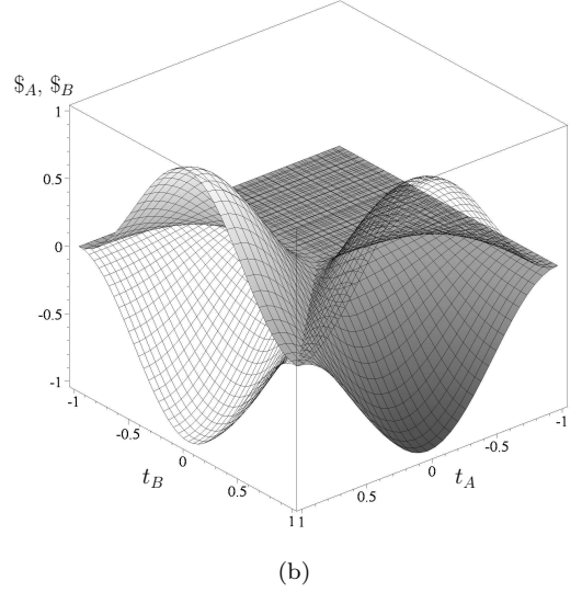
FIG. 5: Expected payoff of scientists A and B in a maximally entangled quantum game ((a): \gamma = \frac{\pi}{2} ) and in a partially entangled quantum game ((b): \gamma = \frac{\pi}{4} ). Payoff setting see Table II.
