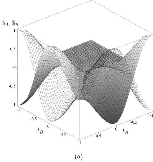
FIG. 5: Expected payoff of scientists A and B in a maximally entangled quantum game ((a): \gamma = \frac{\pi}{2} ) and in a partially entangled quantum game ((b): \gamma = \frac{\pi}{4} ). Payoff setting see Table II.
