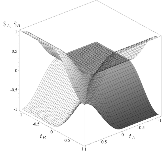
FIG. 4: Expected payoff of scientists A and B in a separable quantum game (payoff setting see Table II).
