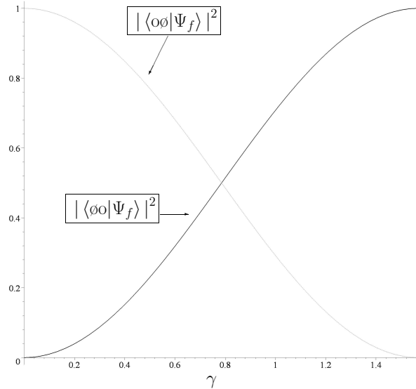
FIG. 13: Joint probabilities of the measurable outcomes as a function of \gamma . Player B chooses strategy \emptyset , whereas Player A chooses \hat{Q} .
