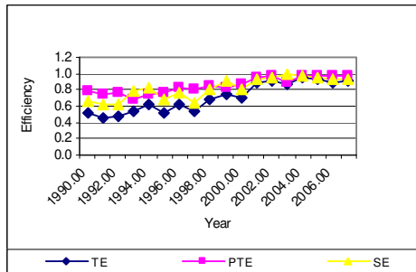
Graph 15: Technical, Pure Technical and Scale Efficiencies-All Banks
