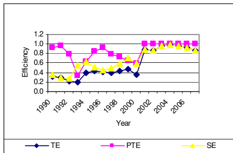
Graph 13: Technical, Pure Technical and Scale Efficiencies-State Banks
