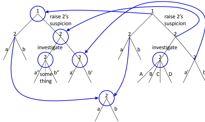
Figure 7: Game form with awareness of unawareness
