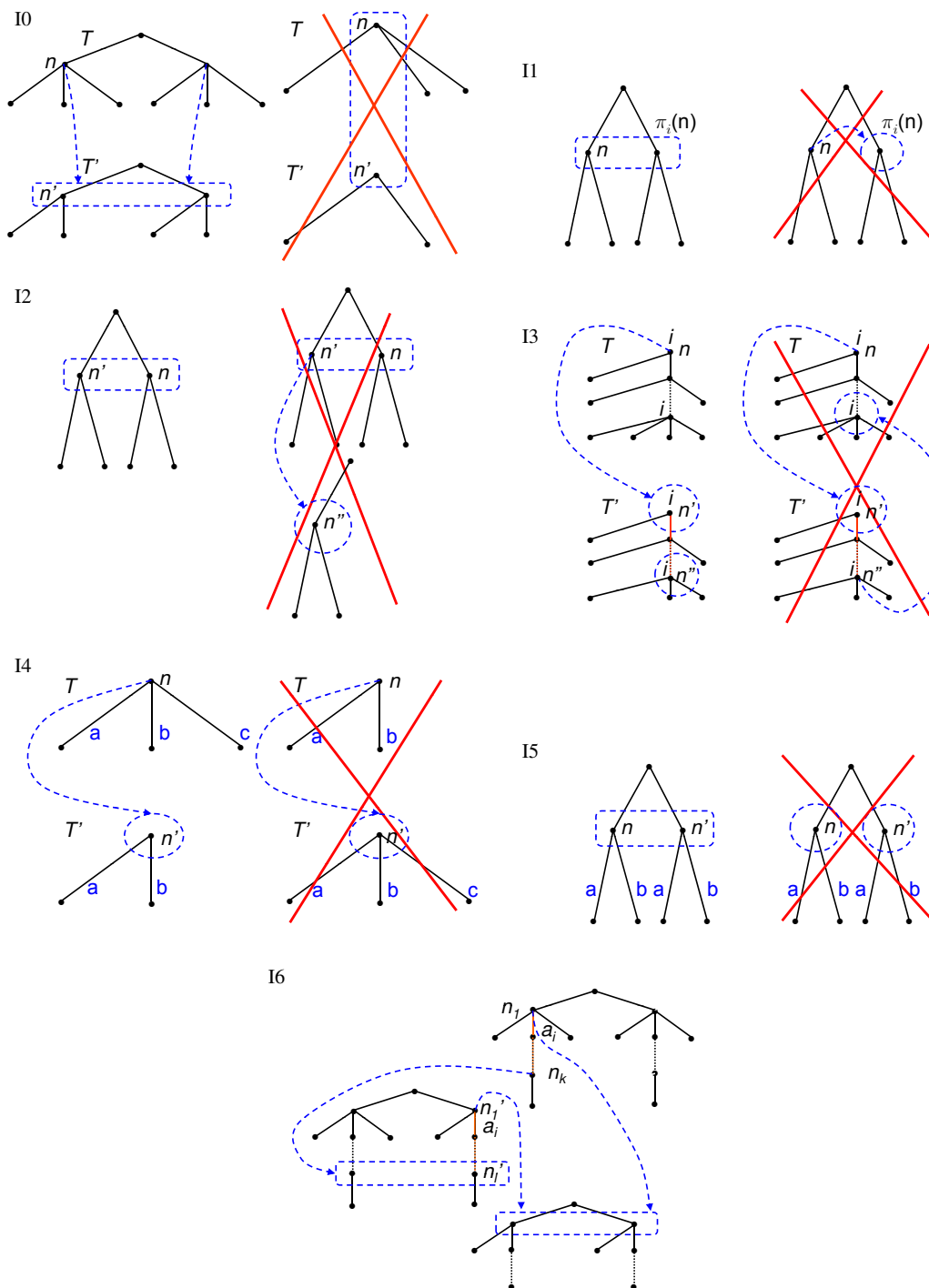
Figure 6: Properties I0 to I6
