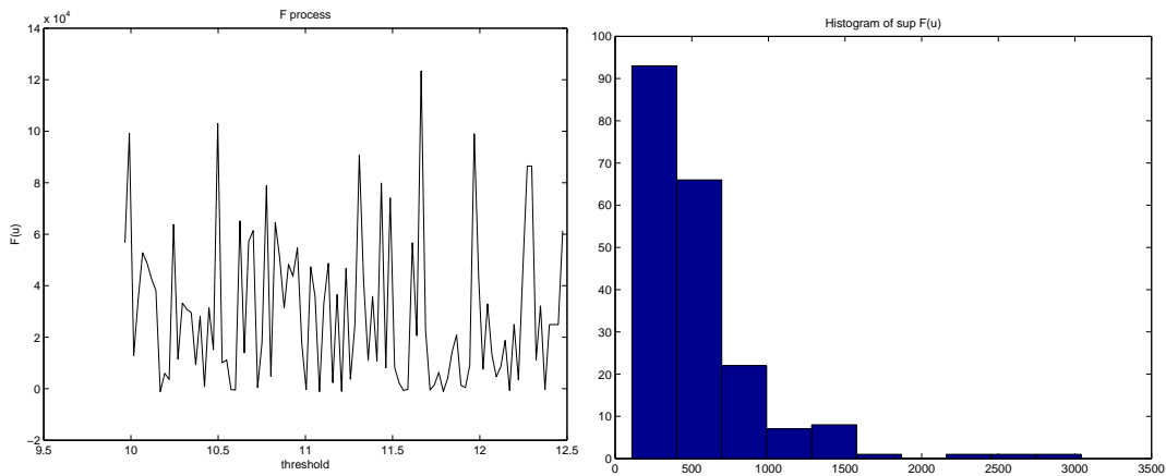
Figure 2. F(\nu) and histogram of the supremum of F(\nu)
