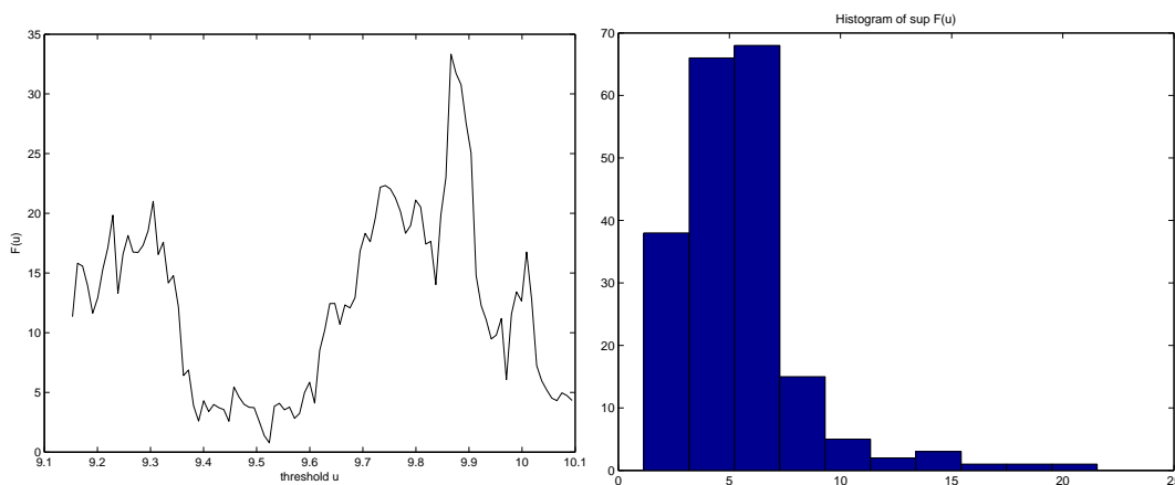
Figure 1. F(u) and histogram of the supremum of F(u)
