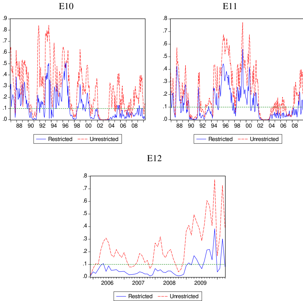
Figure 2: P-values, rolling window from 1979:1-1986:12 to 2002:5-2010:4 30
