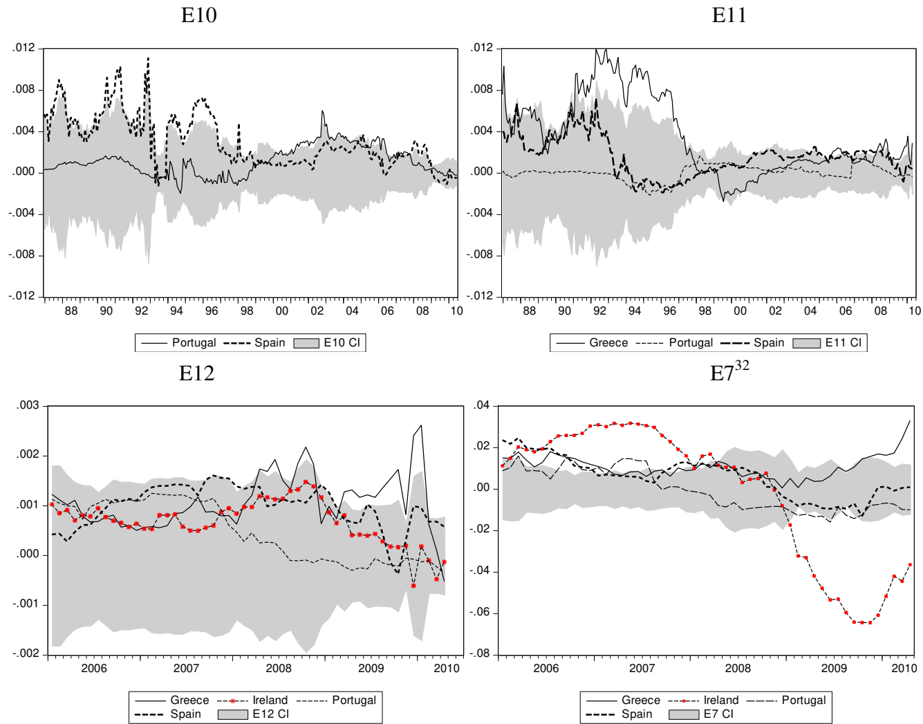
Fig. 5: Individual Deviation Coefficients c_i from the Cross-sectional Mean 31
