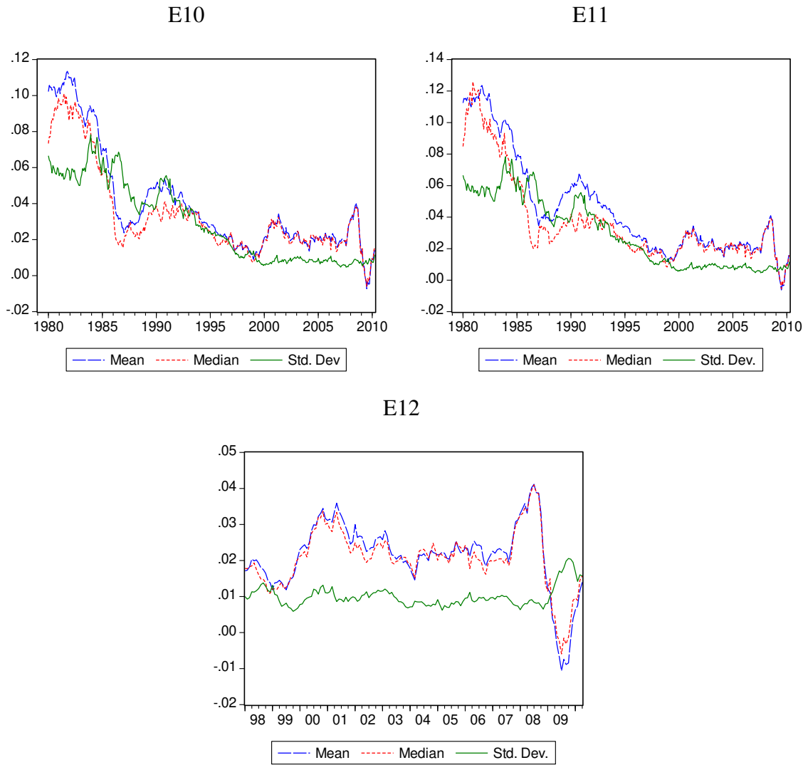
Figure 1: Cross-sectional Mean, Median and Standard Deviation
