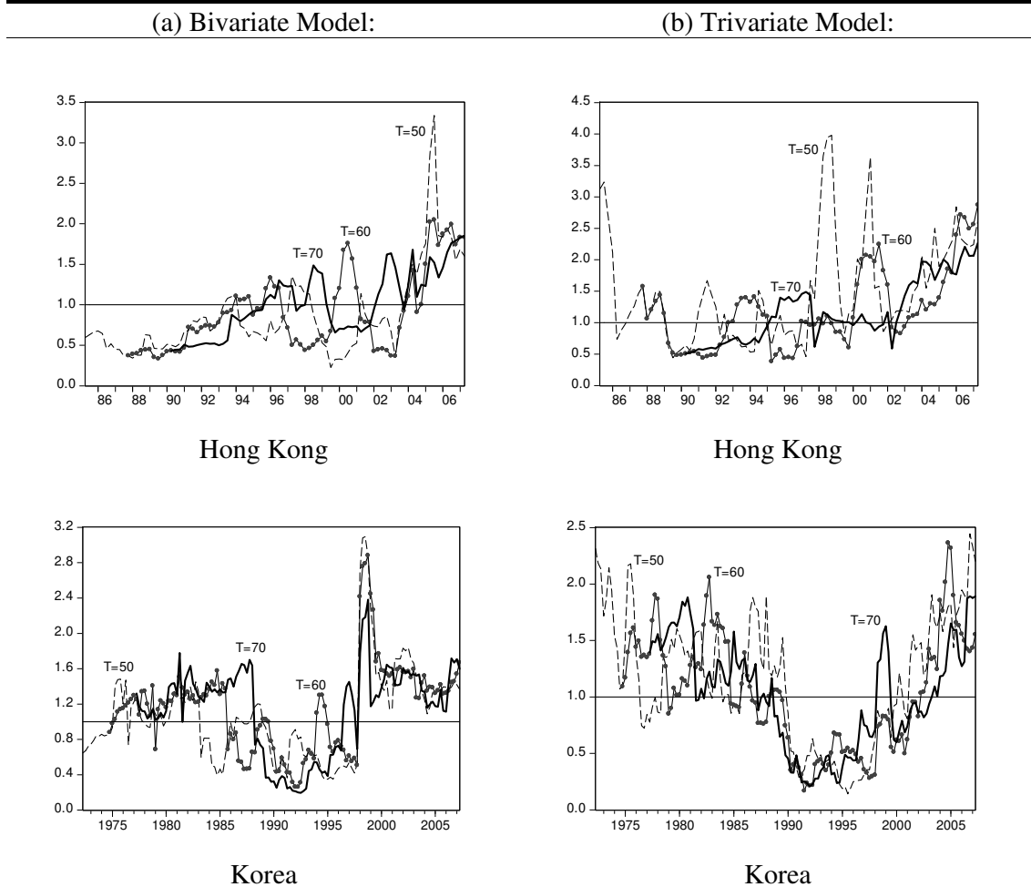
Figure 1: The rolling MWALD causality test
