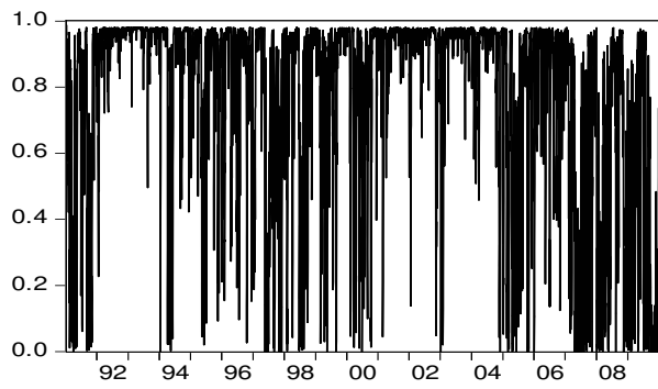
REGIME 1 PROBABILITY
