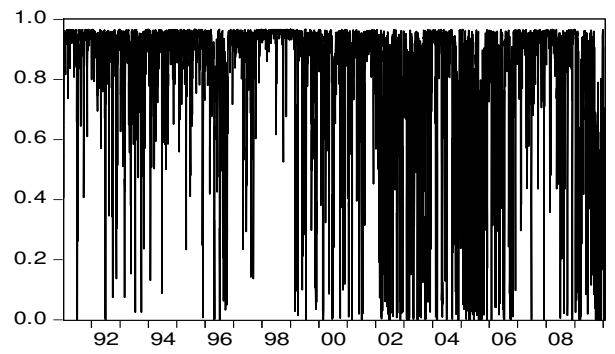
REGIME 1 PROBABILITY
