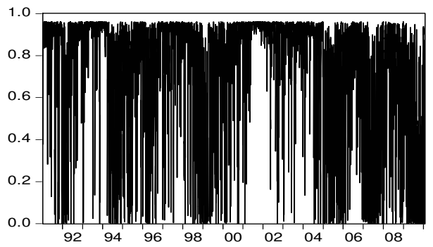
REGIME 1 PROBABILITY
