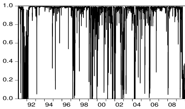
REGIME 1 PROBABILITY
