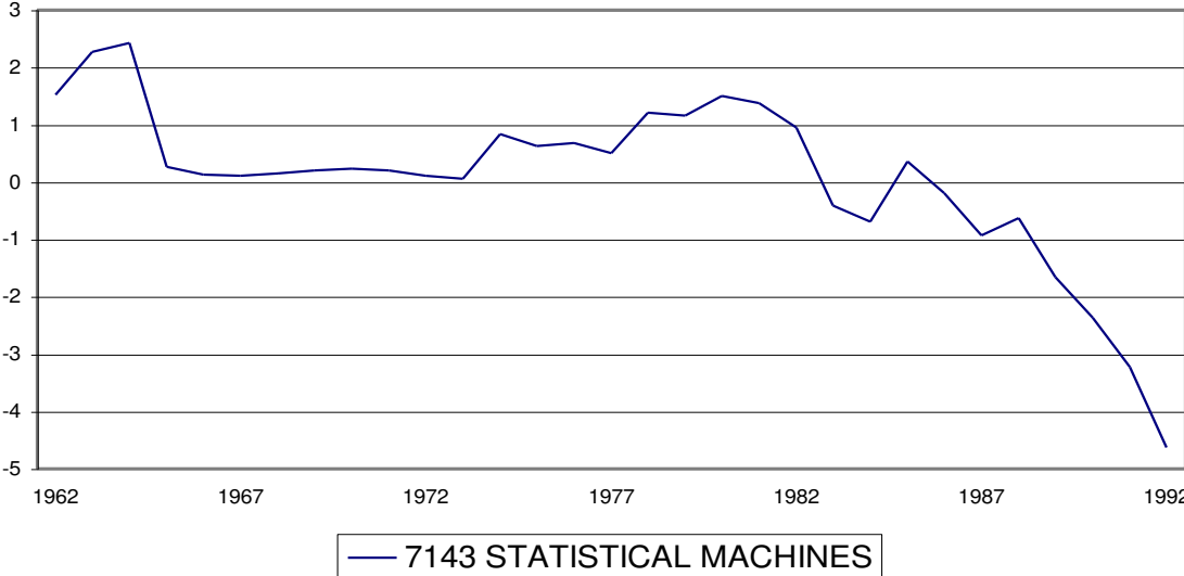
Category VII: ADF Reject, KPSS Fail and Negative Trend
