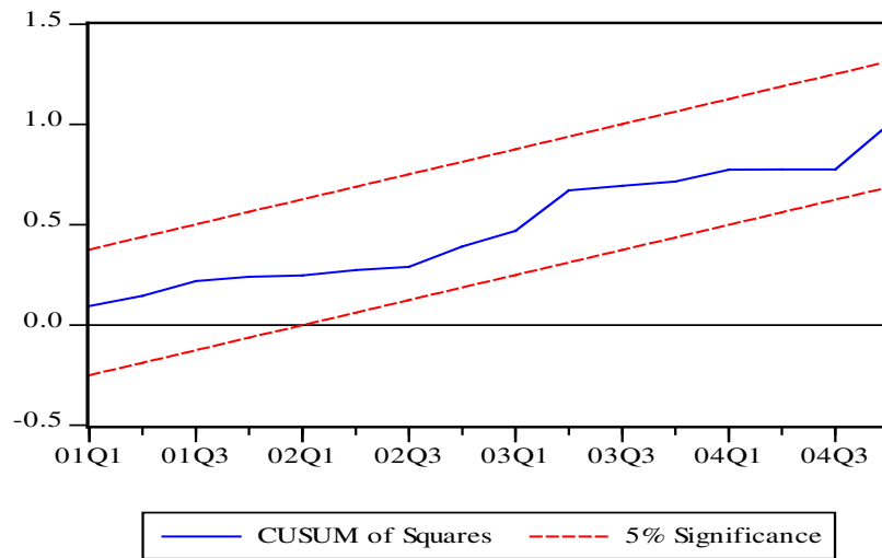
Figure 2: CUSUM of Squares Stability Test for Fiji Stock Market ECM Model
