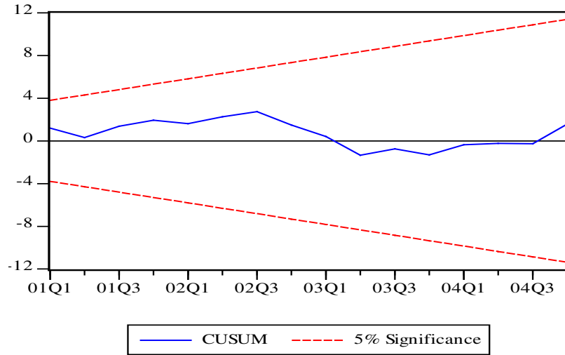
Figure 1: CUSUM Stability Test for Fiji Stock Market ECM Model
