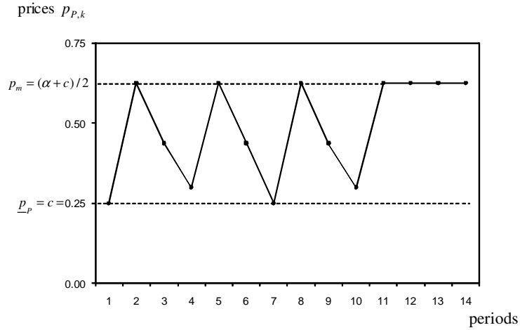
Figure 1: The punishment profile \mathbf{p}_P \equiv (p_P, p_{P,2}, \dots, p_{P,l}) in Example 1 can take the form of asymmetric price cycles (here with \alpha = 1 , c = 1/4 , p_P = p_{NE} = c = 1/4 , implying that \underline{\delta}_M \equiv \sup \{\underline{\delta}, \bar{\delta}\} = 1/2 ). In this ten-period punishment phase, fast price increases from p_P to p_m^* = (\alpha + c)/2 are followed by a two-period fall down to p_P = c (here with intermediate prices a_{P,3} = a_{P,6} = a_{P,9} = (p_P + p_m^*)/2 ).
