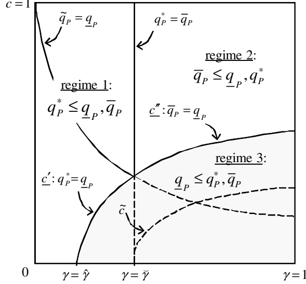
Figure 2: Collusion regimes in plane (c, \gamma) for n \geq 6 . The limited liability constraint binds in the grey area (regime 3). In the benchmark single-period set-up, the collusive quantity is not implementable below the frontier \tilde{c} .
