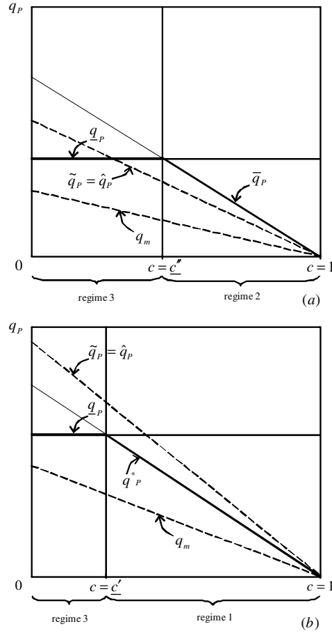
Figure A-3: Thick lines represent optimal punishment quantities (all c , and n \geq 6 ). In (a) products are highly substitutable ( \check{\gamma} < \gamma ). Regime 3 applies for c \leq \underline{c}'' , and regime 2 applies otherwise. In (b) products are more differentiated ( \gamma < \hat{\gamma} ). Regime 3 applies for c \leq \underline{c}' , and regime 1 applies otherwise.
