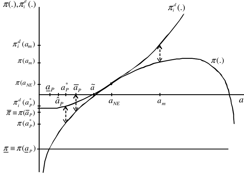
Figure A-1: The optimal punishment action a_P^* is such that \pi_i^d(a_P^*) - \pi(a_P^*) = \pi_i^d(a_m) - \pi_m , given a_m (here with a_P < a_P^* < \bar{a}_P < \tilde{a} ). As in Abreu (1986) the difference \pi_i^d(a_P) - \pi(a_P) is unbounded from above if the limited liability constraint is removed.
