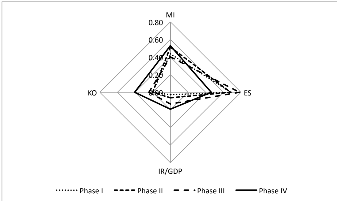
Figure 12: India: Trilemma And Reserves Configuration over time
