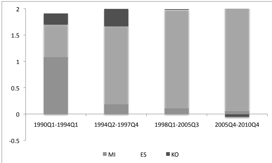
Figure 13: China: Phase-wise Contributions of the Trilemma Policy Objectives
