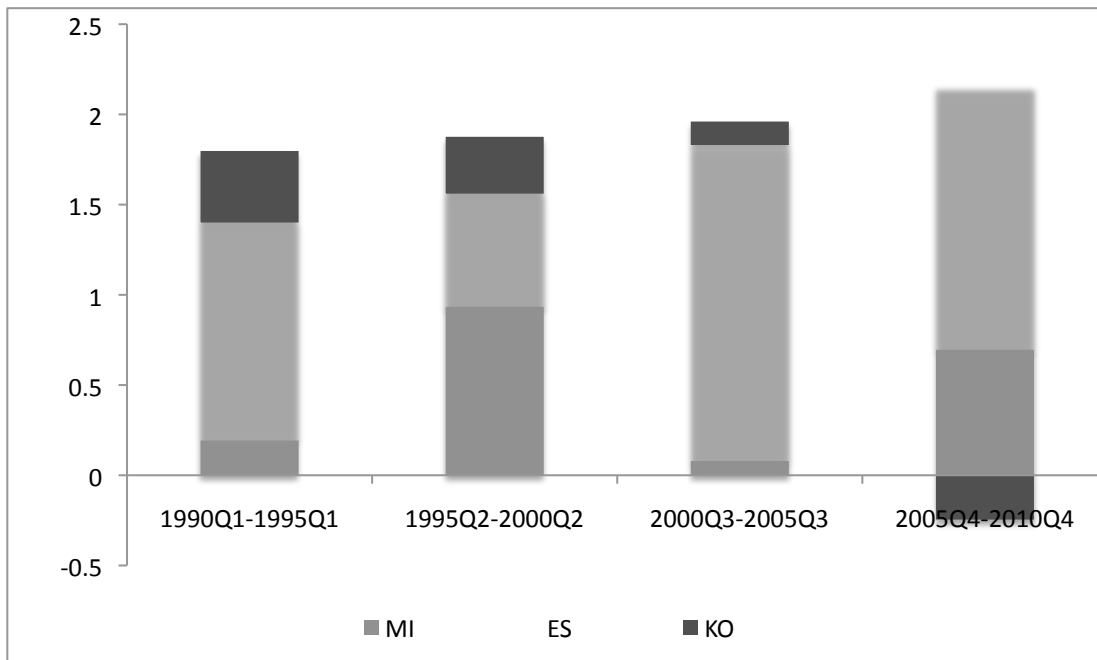
Figure 14: India: Phase-wise Contributions of the Trilemma Policy Objectives
