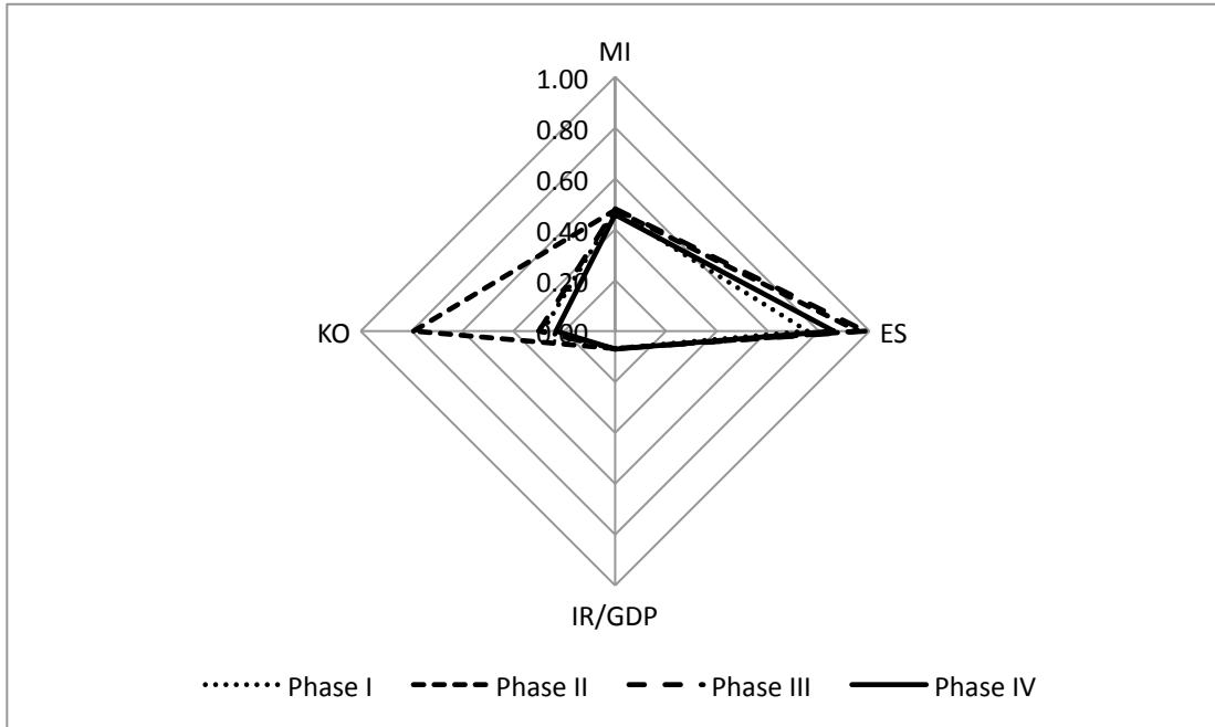
Figure 11: China: Trilemma And Reserves Configuration over time
