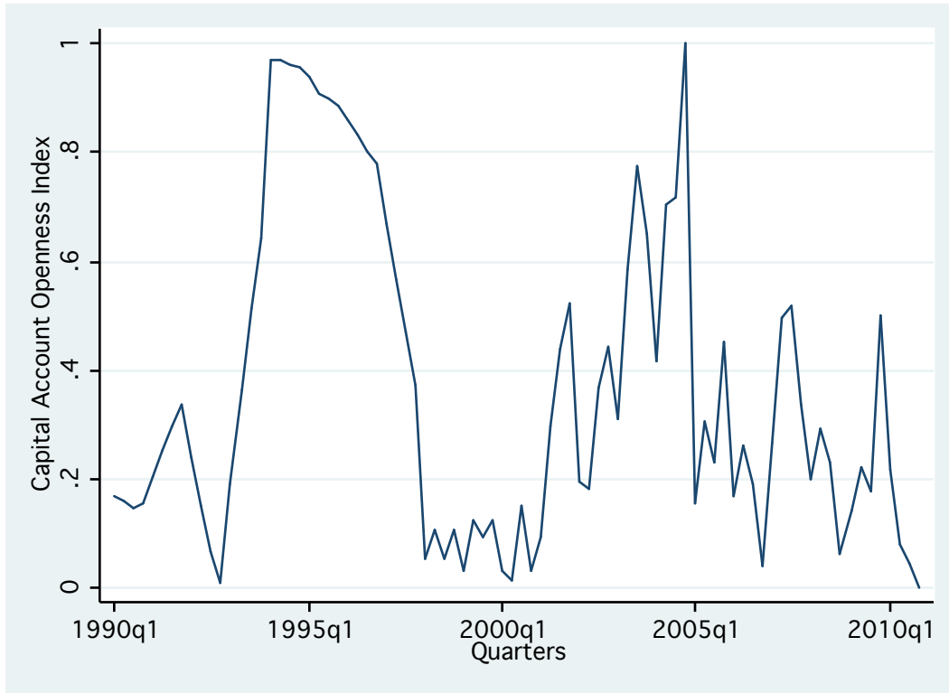
Figure 6: Capital Account Openness Index in India (1990-2010)
