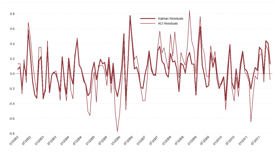
Figure 3: Residual Comparison of ACI and Kalman Approach
