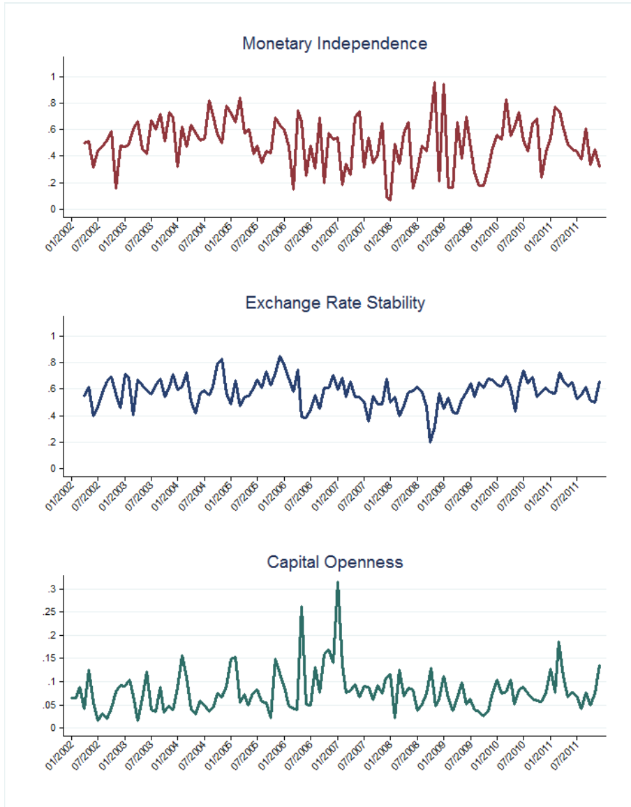
Figure 2: Trilemma Indices
