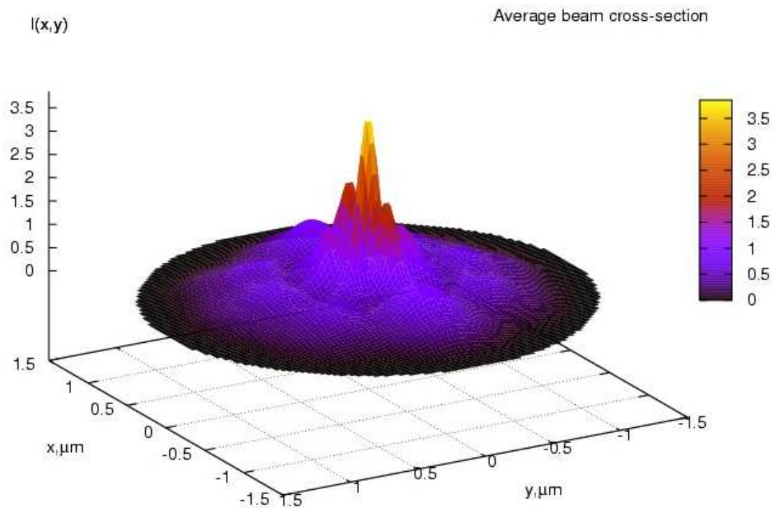
Figure 5: Laser beam transversal distribution (averaged over the whole lasing time period).
