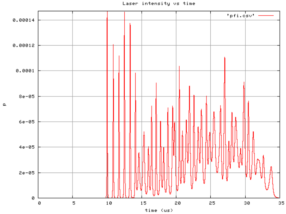
Figure 10: Typical random-pulsed lasing
